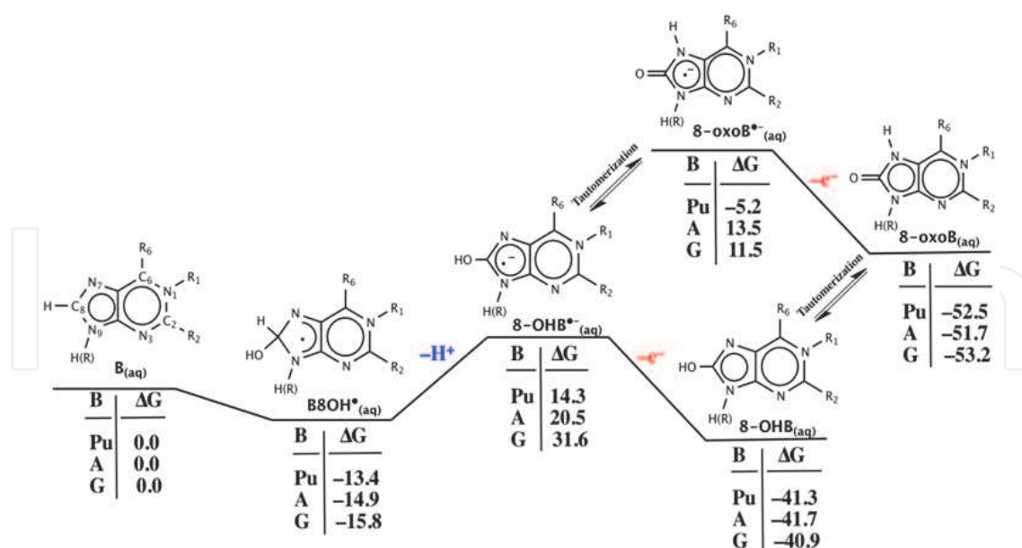
Fig. 3. Calculated (see text) standard Gibbs energies (kcal mol -1 ) for PT initiated oxidation of B8OH•.
