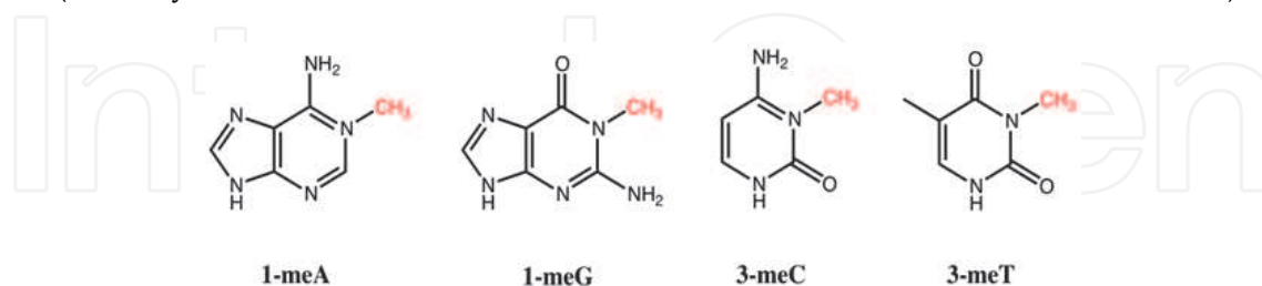
Fig. 8. Examples of methylated substrates that are dealkylated by the AlkB family of enzymes. The methyl groups to be removed have been colored in red.
