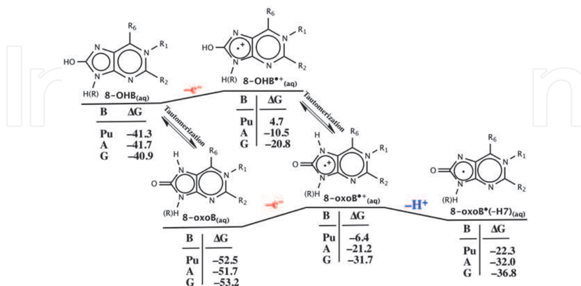
Fig. 5. Calculated (see text) standard Gibbs energies (kcal mol -1 ) for oxidation of 8-OHB and 8-oxoB .
