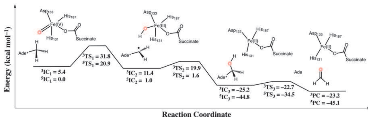
Fig. 9. Potential energy surface for the demethylation of the methylated adenine nucleobase model 3me4amPym + in the triplet and quintet spin states.
