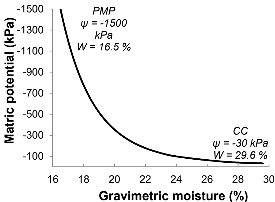
Fig. 3. Moisture retention curve in the experimental site.
