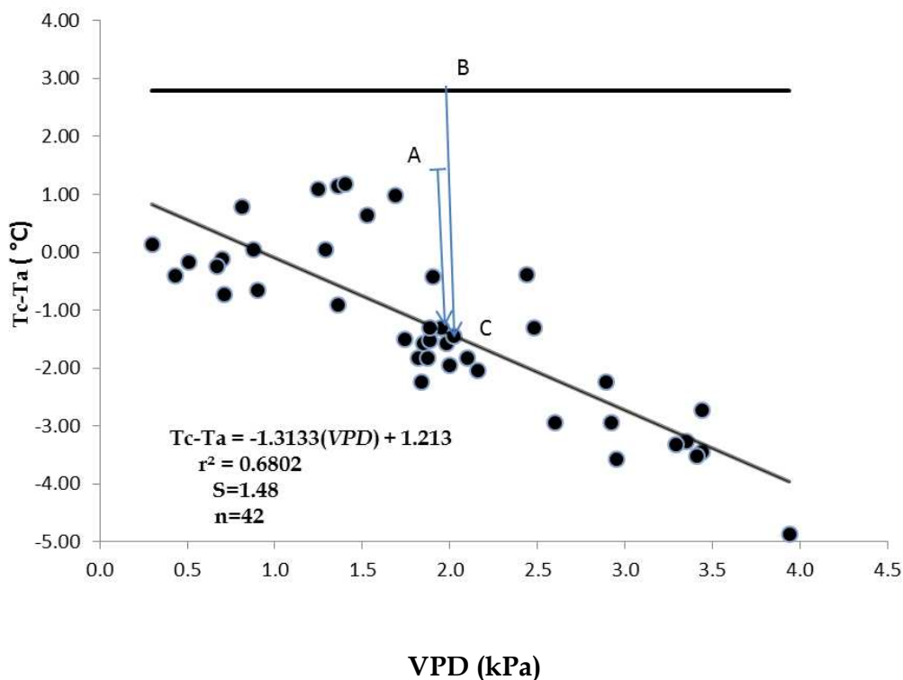
Fig. 5. The lower (A-C) and upper (B-C) baselines for husk tomato crop for determining the crop water stress index. S = Standard deviation.
