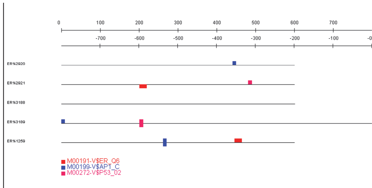
Fig. 3. ER, AP-1 and p53 binding motifs relative to miR-342, miR-21 and miR-143~145. The red, blue and pink boxes represent ER, AP-1 and p53 binding sites respectively. ER_2920 and ER2921 located in miR-342 upstream region; ER_3188 and ER_3189 located in miR-21 regulatory region; ER_1259 located in miR-21 upstream region (please referring to Figure 1).
