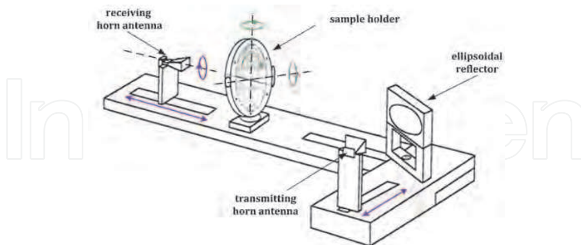
Fig. 7. Schematic diagram of the free space setup for the experimental determination of the rotation angle and the three constitutive parameters of isotropic chiral material in the X-Band (not to scale).
