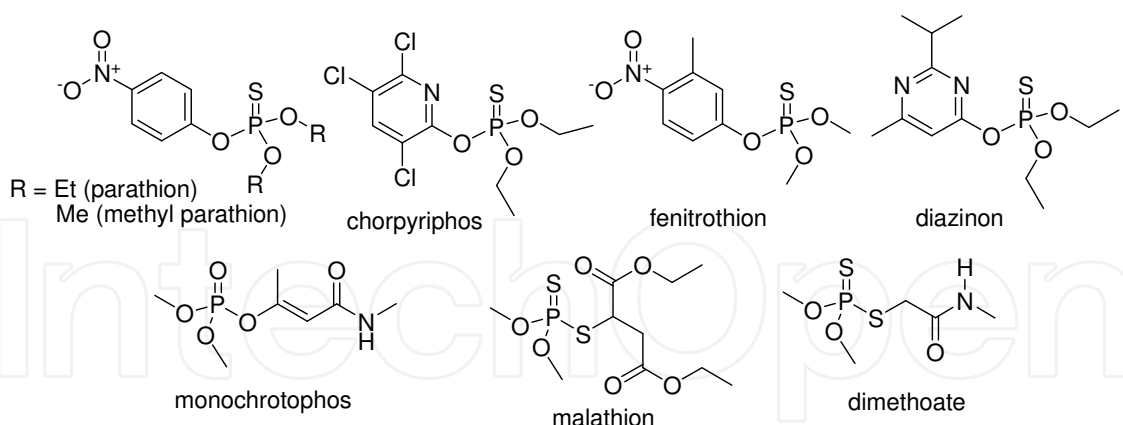
Fig. 4. Structures of organophosphate pesticides
