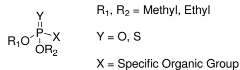
Fig. 3. General structure of organophosphate pesticides
