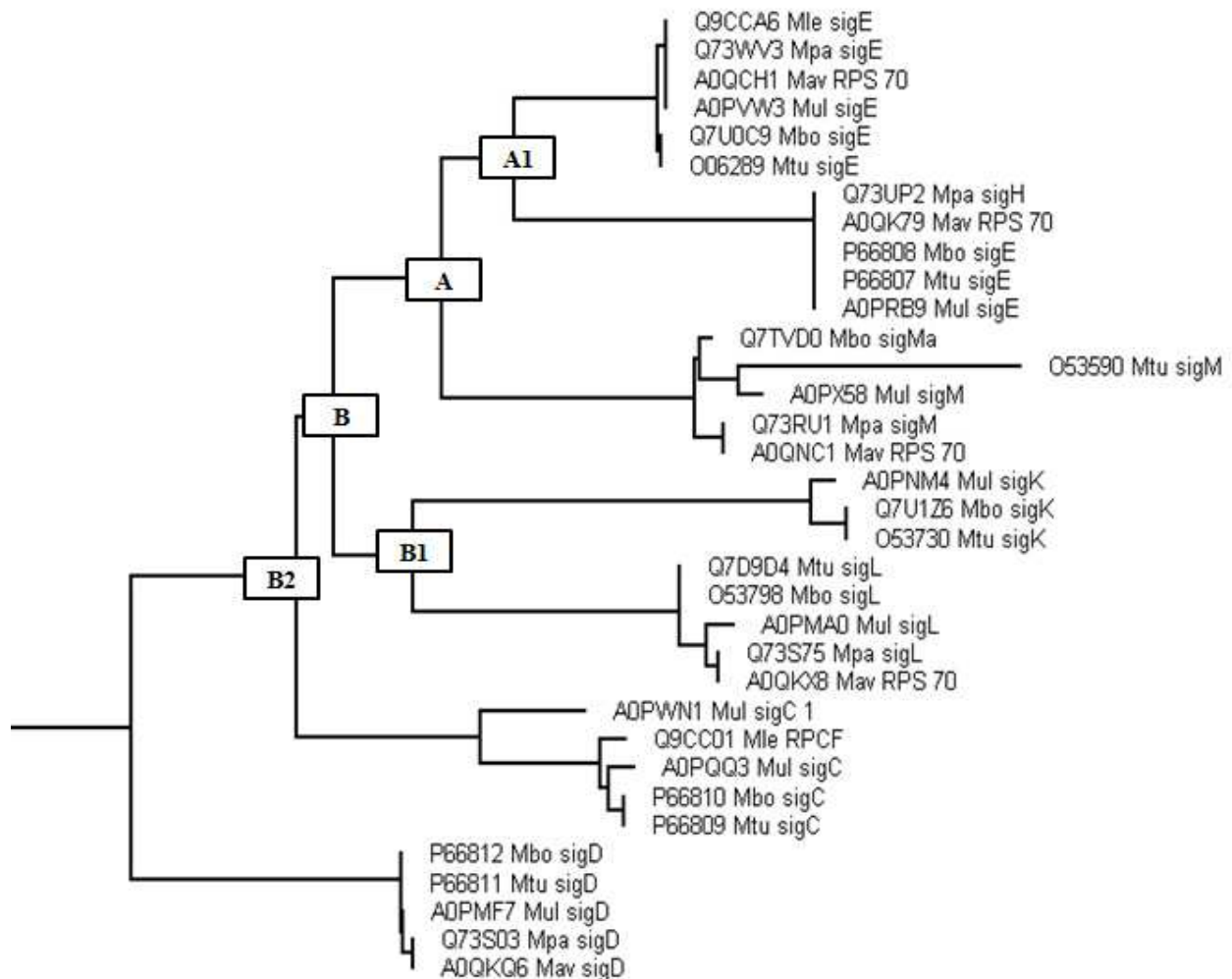
Fig. 12. Phylogenetic tree of the Sigma factor ortholog and paralog cluster inferred by the maximum likelihood method. The duplication events are marked by A's and B's. The labels Mtu, Mbo, Mav, Mul, Mpa and Mle represent proteins from M. tuberculosis , M. bovis , M. avium , M. ulcerans , M. paratuberculosis and M. leprae respectively.
