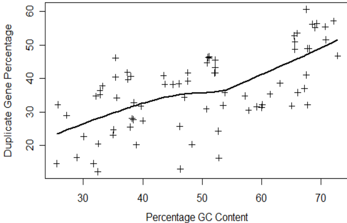
Fig. 1. Scatter plot analysis of the relationship between GC content and duplicate gene percentages of the selected organisms. The percent GC content is plotted on the X-axis and duplicate gene percentage on the Y-axis. The graph suggests that a positive correlation between GC content and duplicate gene percentages exists for the majority of the investigated organisms.
