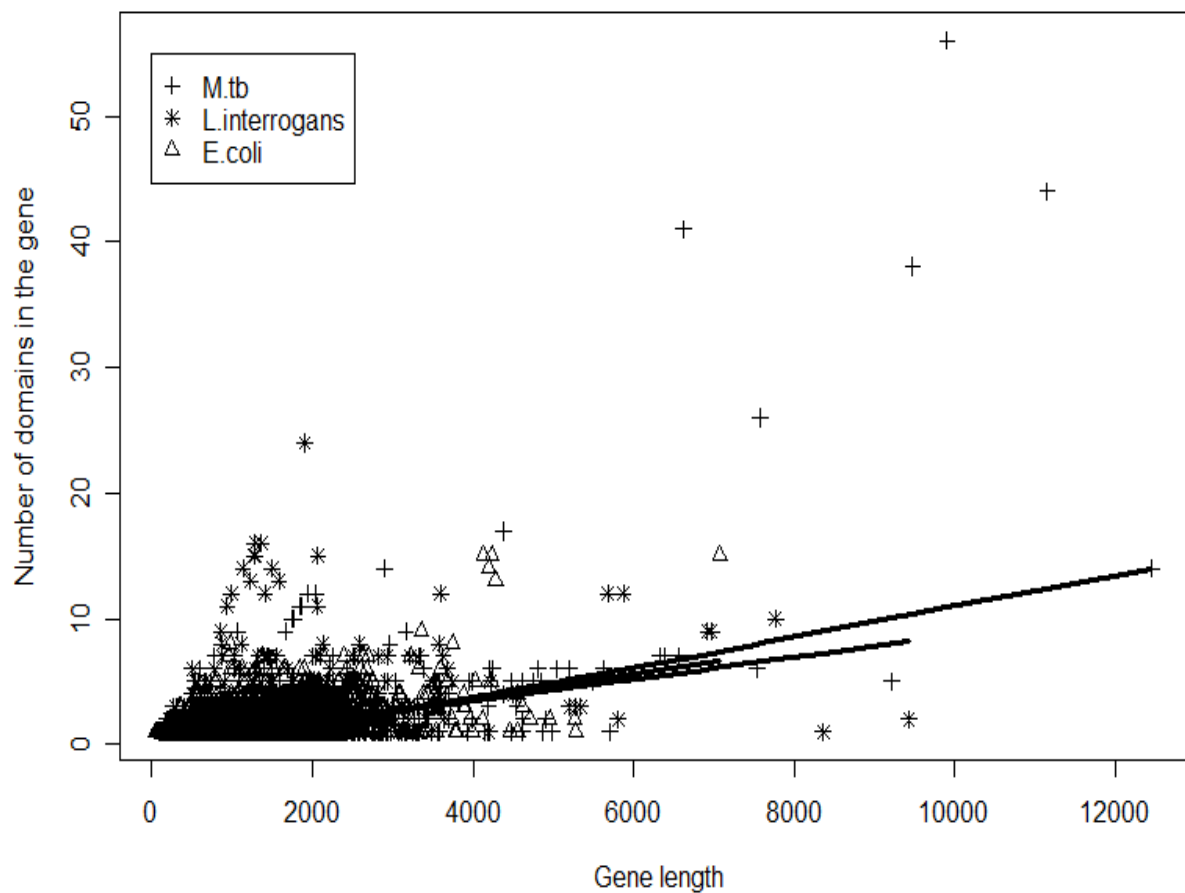
Fig. 5. Investigation of number of domains per gene in the M. tuberculosis H37Rv, E. coli and L. interrogans genomes (Whole Genome Analysis). The graph displays the relationships between gene length and number of domains. The sequence lengths of each gene are plotted on the X-axis and the corresponding number of domains per gene on the Y-axis. From the graph, it can be inferred that the gene length is not necessarily dependent on domain number.
