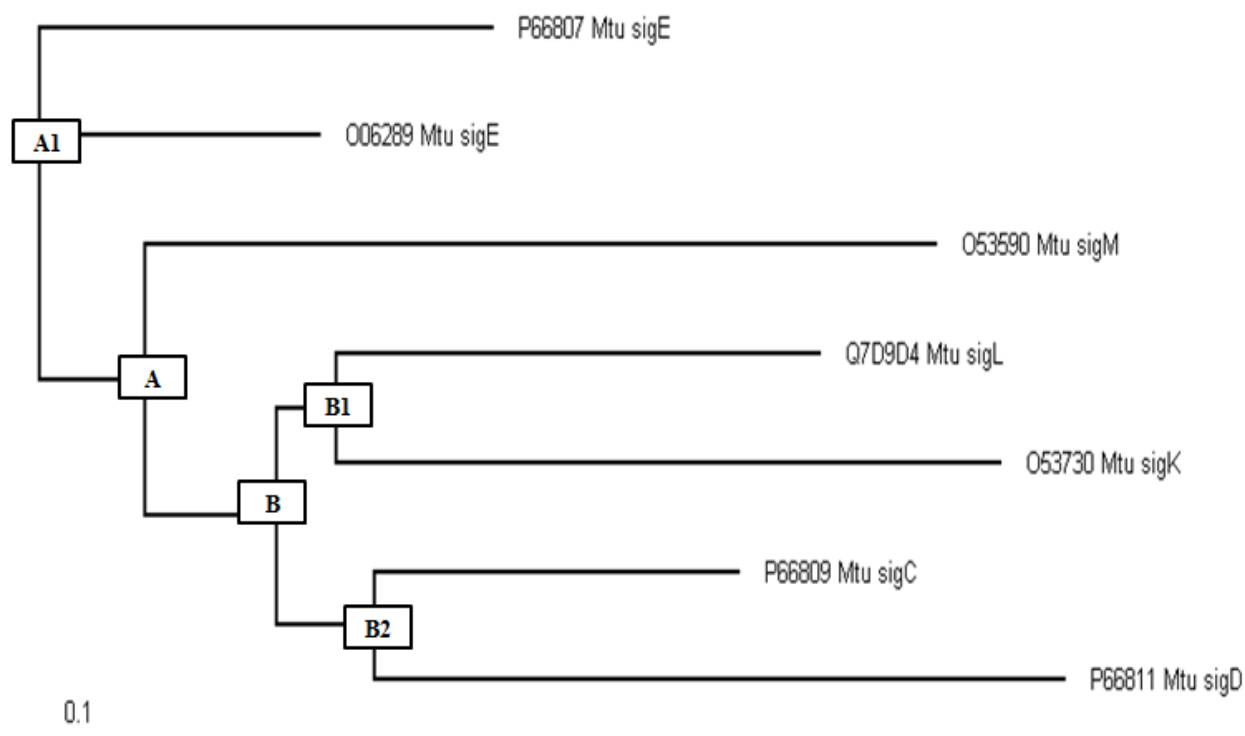
Fig. 11. Phylogenetic tree of the Sigma factor paralog cluster inferred by the maximum likelihood method. The duplication events are marked by A's and B's. The figure displays the phylogenetic diversification of sigma factors (sigE, sigM, sigL, sigK, sigC and sigD).
