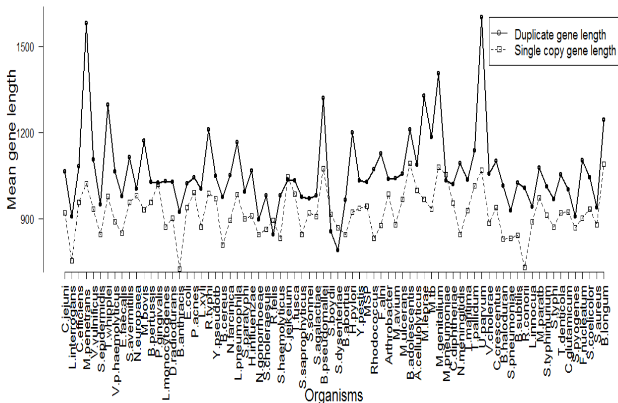
Fig. 3. Comparison of Functional Complexity of the Expanded and Single Copy Gene Families Based on Nucleotide Sequence Data. The graph displays the mean gene lengths of duplicate and single copy genes in the investigated organisms. The organisms are plotted on the X-axis and the corresponding mean gene length on the Y-axis.
