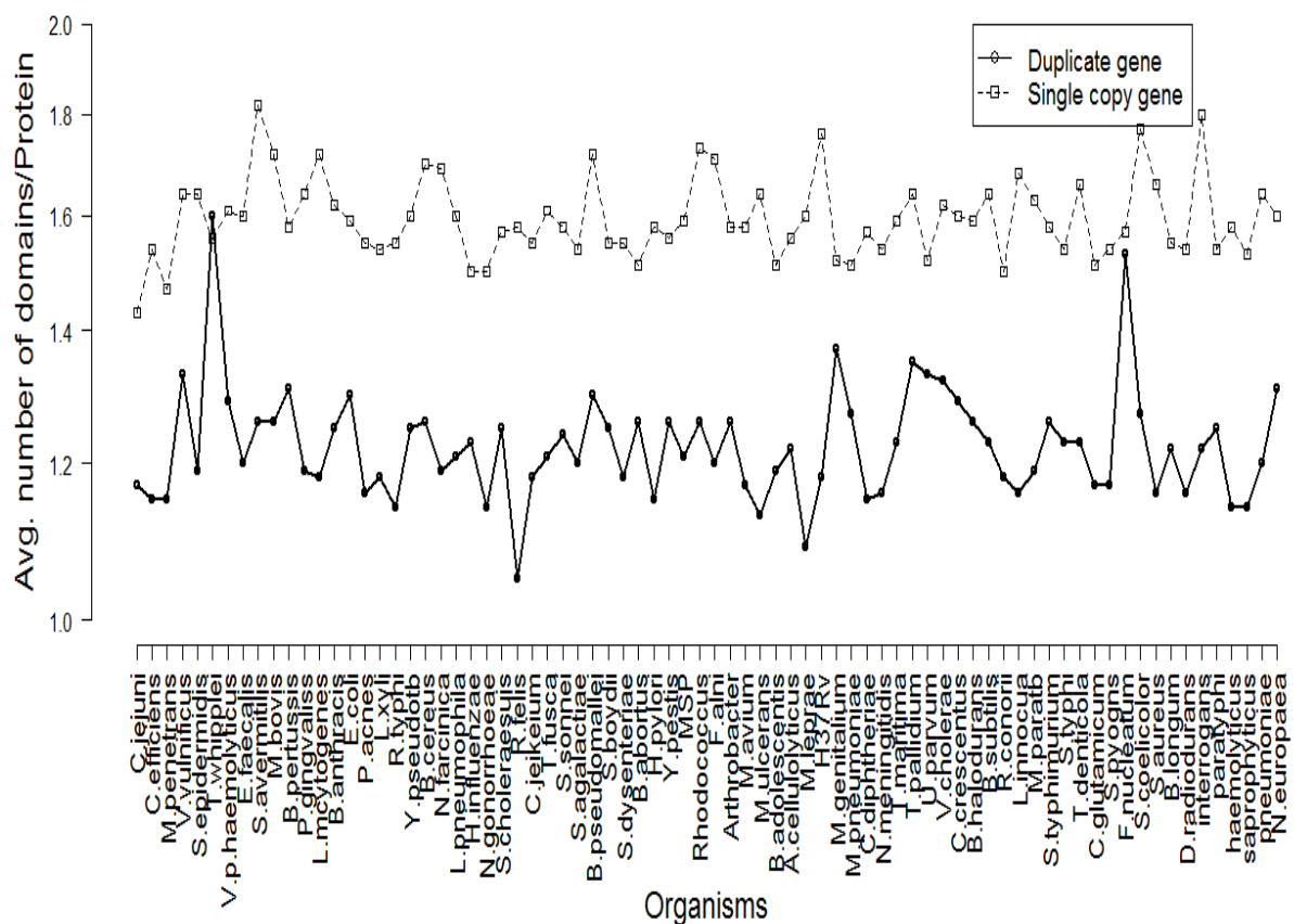
Fig. 4. Comparison of Functional Complexity of the Expanded and Single Copy Genes Based on InterPro Signature Data in Selected organisms. The graph displays the mean number of domains per protein in the duplicate and single copy genes of each organism. The organisms investigated are plotted on the X-axis and the corresponding mean number of domains per protein for each organism on the Y-axis.
