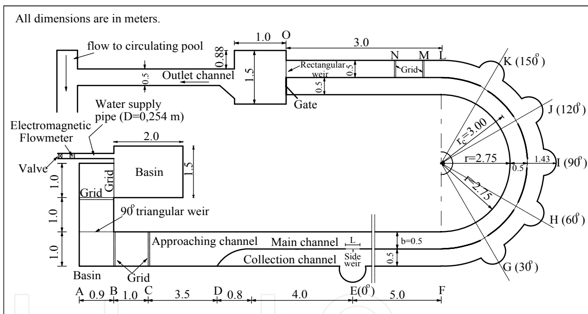
Fig. 2. Experimental arrangement.
