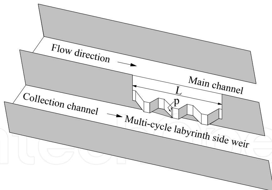
Fig. 11. Trapezoidal labyrinth side weir with multi-cycle.
