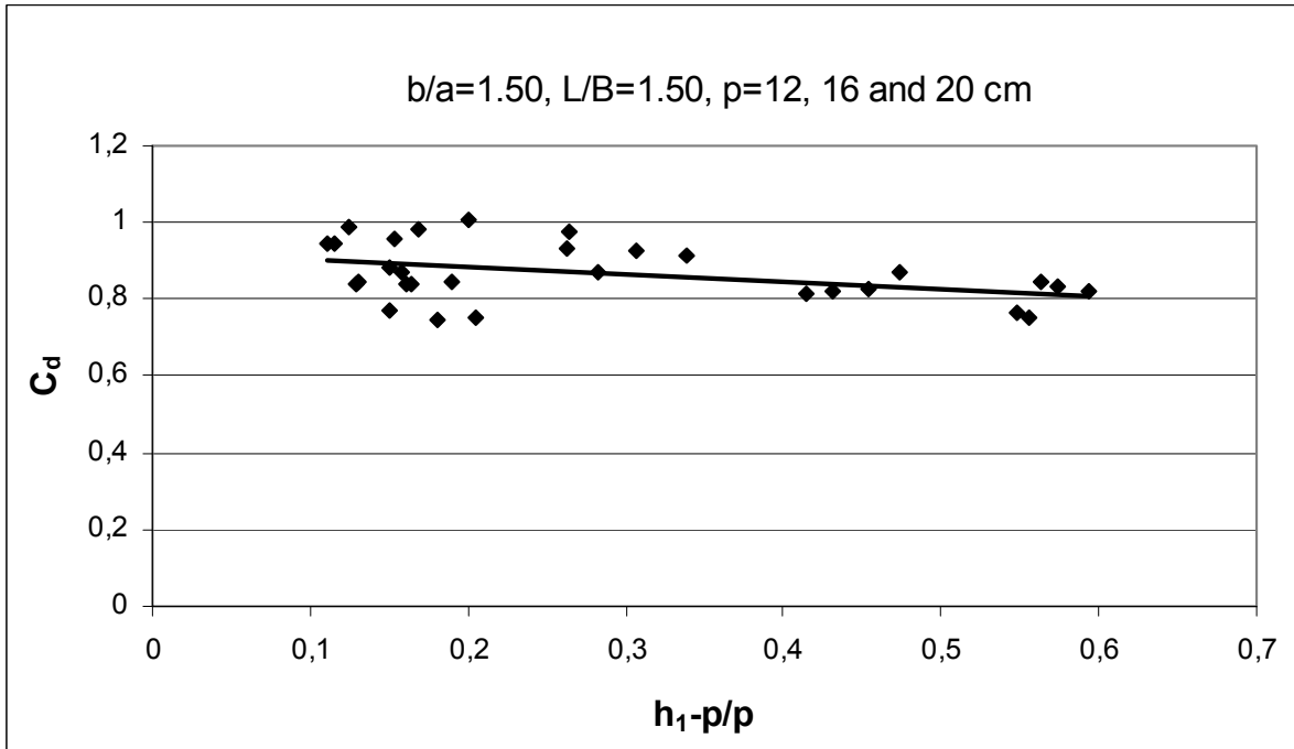
Fig. 16. Variation of C_d versus h_1-p/p for \alpha=16^\circ .
