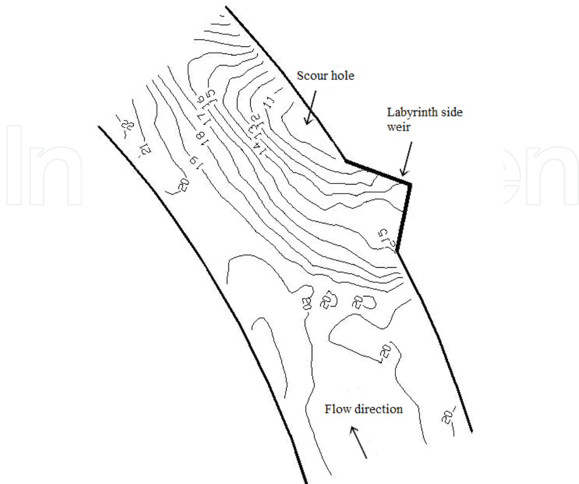
Fig. 23. Bed topography at a side weir intersection when \alpha=30^\circ , \theta=90^\circ , V/V_c=0.8214 , L/B=0.50 and p/B=0.32 (contours in cm and undisturbed bed level is 20 cm).
