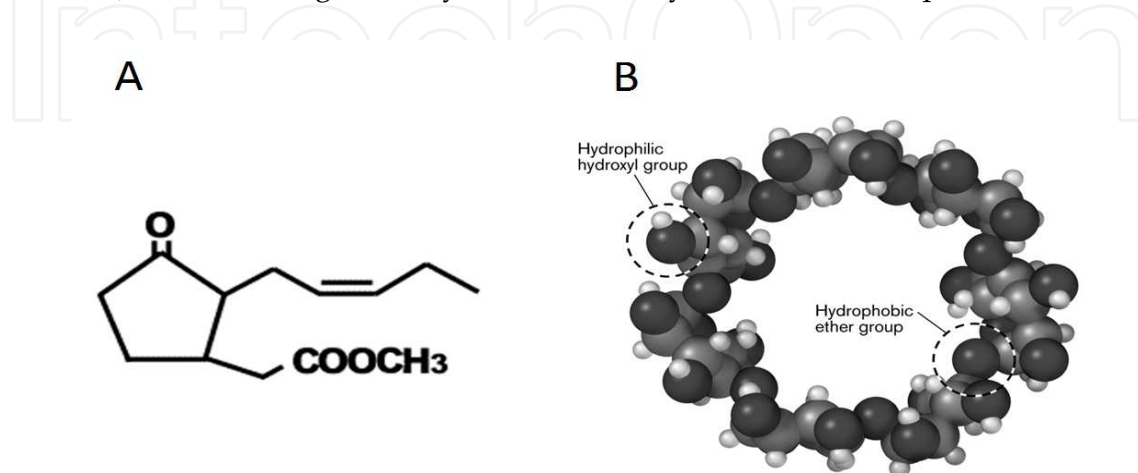
Fig. 3. Structures of methyl jasmonate (A) and cyclodextrins (B).
