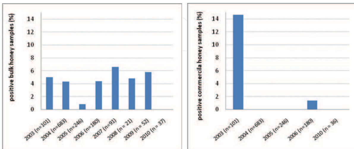
Fig. 2. Residues of volatile insecticides in Greek honeys
