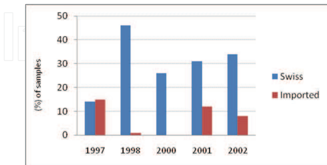
Fig. 1. Residues of p-DCB in honey samples in Switzerland (Bogdanov et al., 2004)
