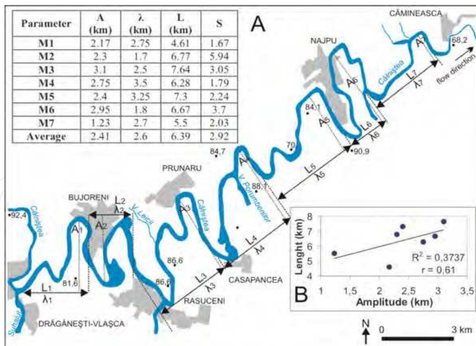
Fig. 11A. The meander morphometry of the Câlniștea River (according to Greu et al., 2010b, modified). B. Corellation between the length and the amplitude of the meanders of the Câlniștea River in the study reach. M1...M7: meander number; A: meander amplitude; \lambda : meander wavelength; L: channel length; S: sinuosity ratio.
