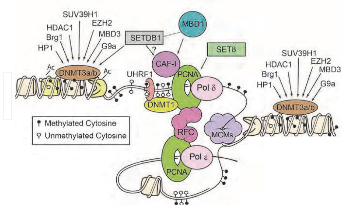
Fig. 2. Propagation of DNA methylation. Hemimethylated cytosines on newly synthesized DNA are recognized by UHRF1 (pink). The unmethylated daughter strand is methylated by the maintenance methyltransferase, Dnmt1, (yellow) which is localized to the replication fork through interactions with PCNA (bright green) and UHRF1. Dnmt3a/3b (brown) are de novo methyltransferases that localize to nucleosome-bound DNA and also interact with UHRF1 (not shown). Factors interacting with Dnmt3a/3b, include heterochromatin protein HP1, chromatin remodeler Brg1, histone deacetylase HDAC1, H3 K9 methyltransferases SUV39H1 and G9a, H3 K27 methyltransferase EZH2 and methyl DNA binding protein MBD3. The H3 K9 methyltransferase SETDB1 (grey) also interacts with Dnmt3a/3b and is localized to the replication fork through the chromatin assembly factor CAF-1 (magenta). CAF-1, which binds PCNA, also recruits the methyl DNA binding protein MBD1 (teal) that directly interacts with SETDB1. The mechanism for interaction between SETDB1 and CAF-1 is unclear and denoted by the question mark. The H4 K20 methyltransferase SET8 (dark green) is also targeted to the replication fork through interactions with PCNA.
