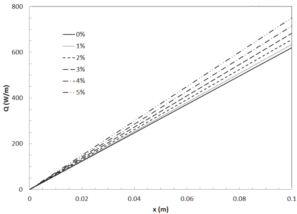
Fig. 19. Thermal flow rate for Alumina / water nanofluid
