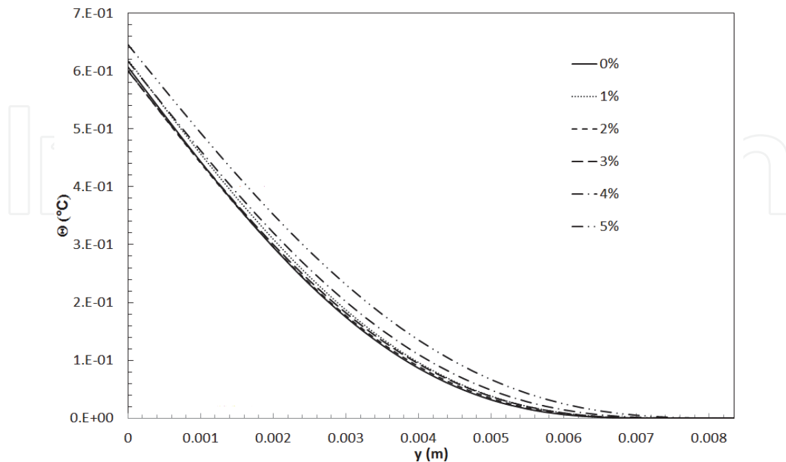
Fig. 8. Temperature profiles at x = 0.1\text{ m} abscissa for CuO / water nanofluid
