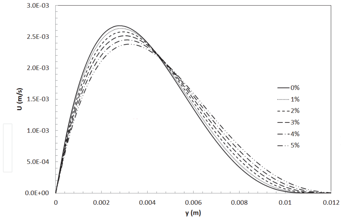
Fig. 5. Velocity profiles at x = 0.1 m abscissa for Alumina / water nanofluid
