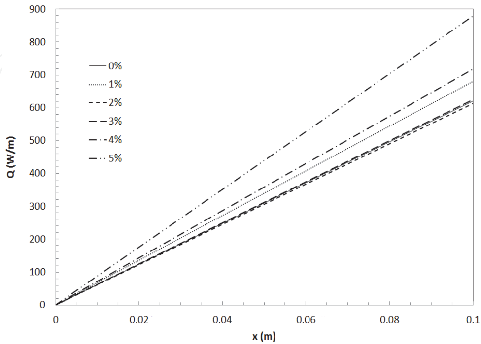
Fig. 18. Thermal flow rate for CuO / water nanofluid
