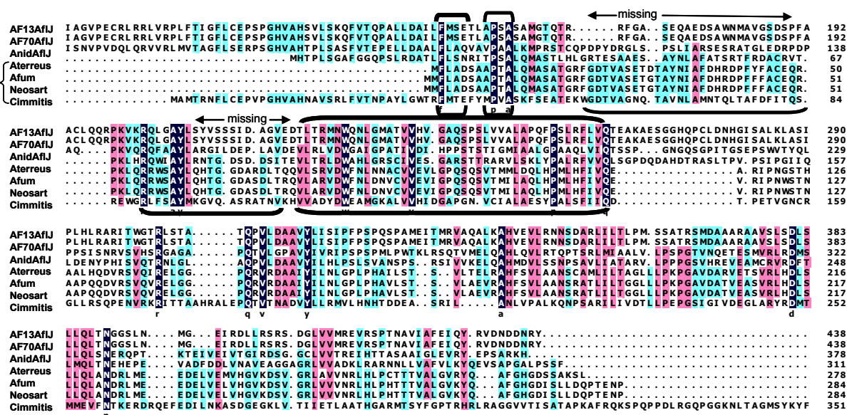
Fig. 4. Comparison of A. flavus AflJ sequence to those of non-aflatoxin producing species reveals partial homology to methyltransferase-2 family proteins. The bracketed proteins have O-methyltransferase domains. Regions bracketed at the bottom are the predicted methyltransferase domains.
