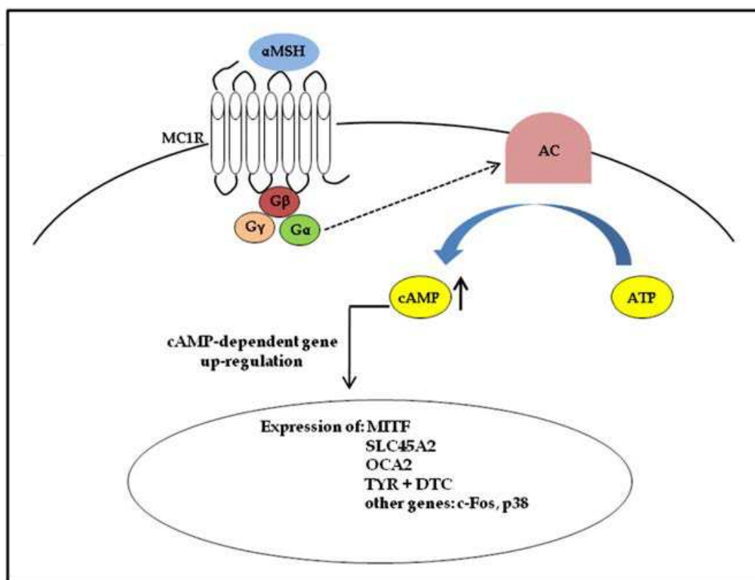
Fig. 3. MSH-MC1R signalling pathway.
