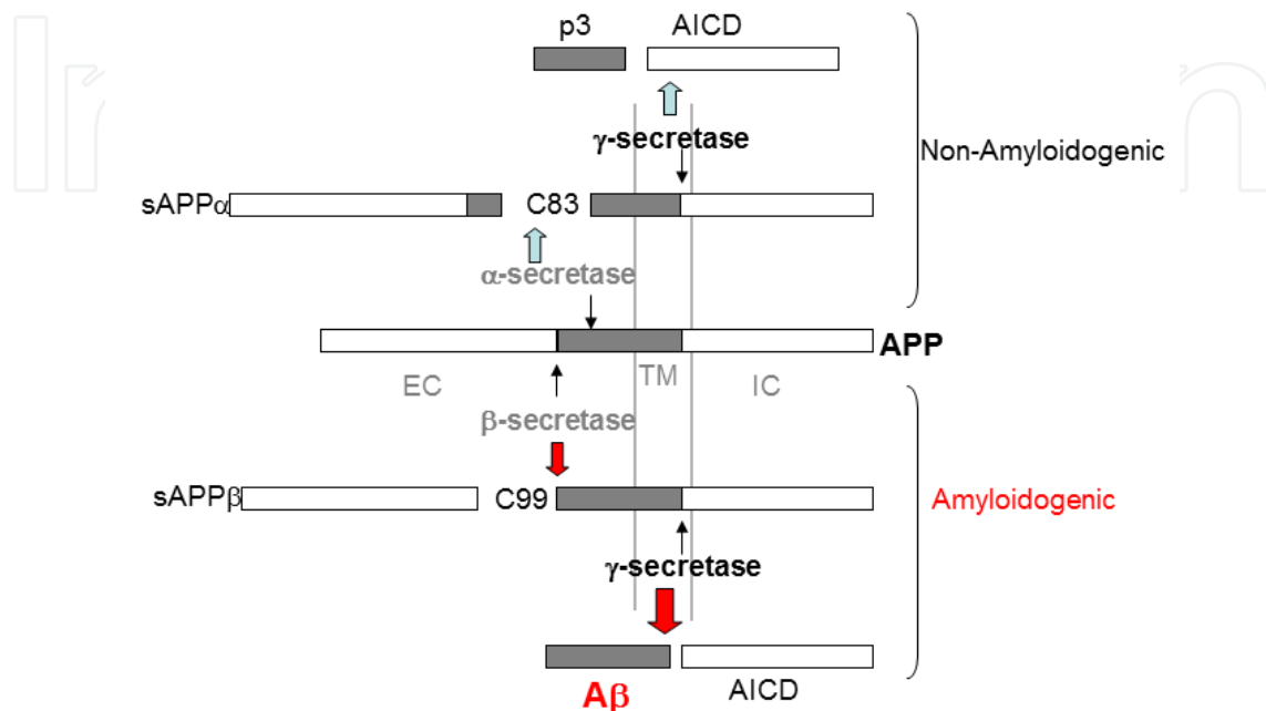
Fig. 1. Schematic diagram of APP processing (not drawn in scale). TM-transmembrane; EC-extracellular; IC- intracellular
