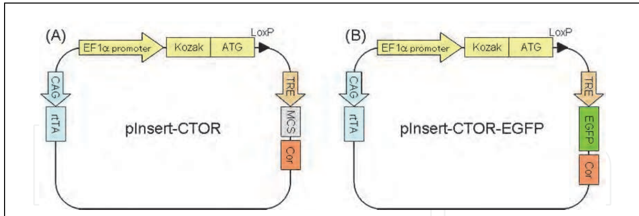
Fig. 5. (A) pInsert-CTOR and (B) pInsert-CTOR-EGFP vectors for the first-generation Tet-inducible gene expression system based on the site-directed integration.
