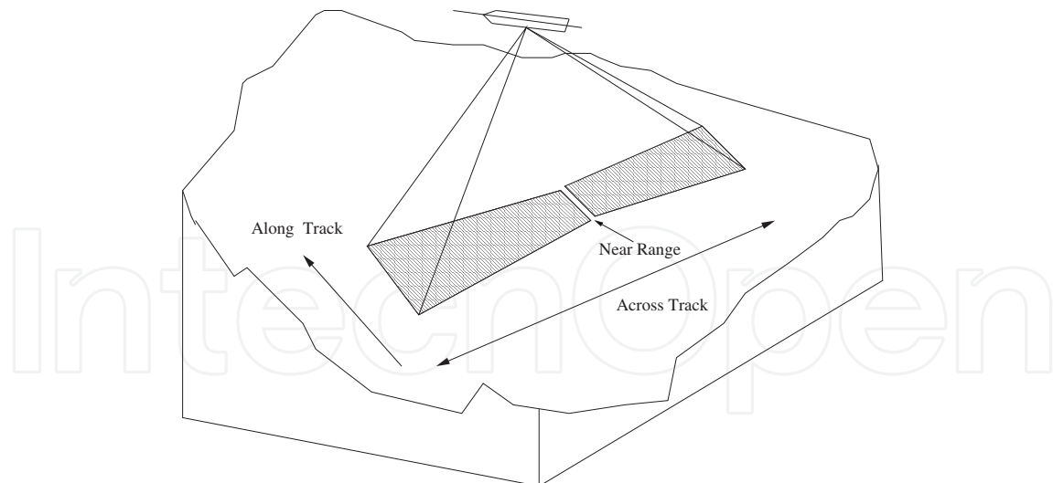
Fig. 2. Schematic diagram of the acoustic 'footprint' of a side-scan sonar system. The gray area represents the swath
