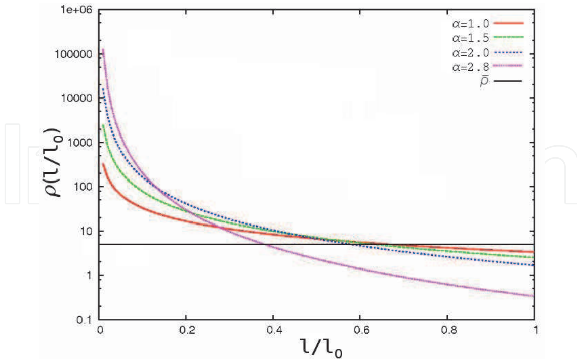
Fig. 3. Dependence of \rho for different values of \alpha . The black solid line represents the case of a homogeneous density \bar{\rho}
