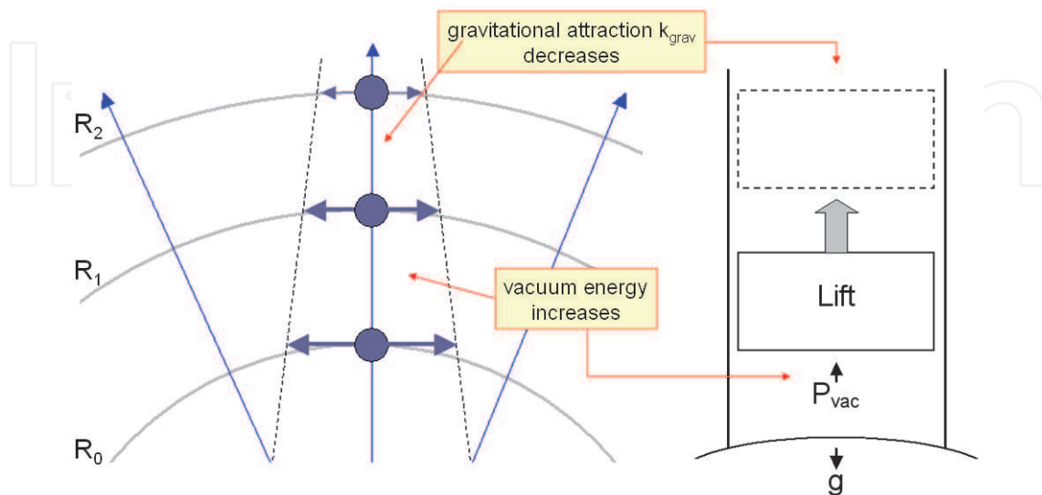
Fig. 1. Schematic illustration of the physical action of a constant vacuum energy density and of inter-material cosmic gravitational fields requiring work to be done, if co-moving matter is transferred to larger cosmic scales S = R .
