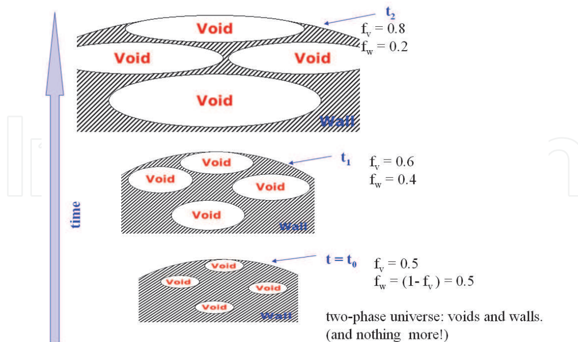
Fig. 4. Illustration of the non-homologous expansion of a two phase universe with void and wall regions having different matter densities.
