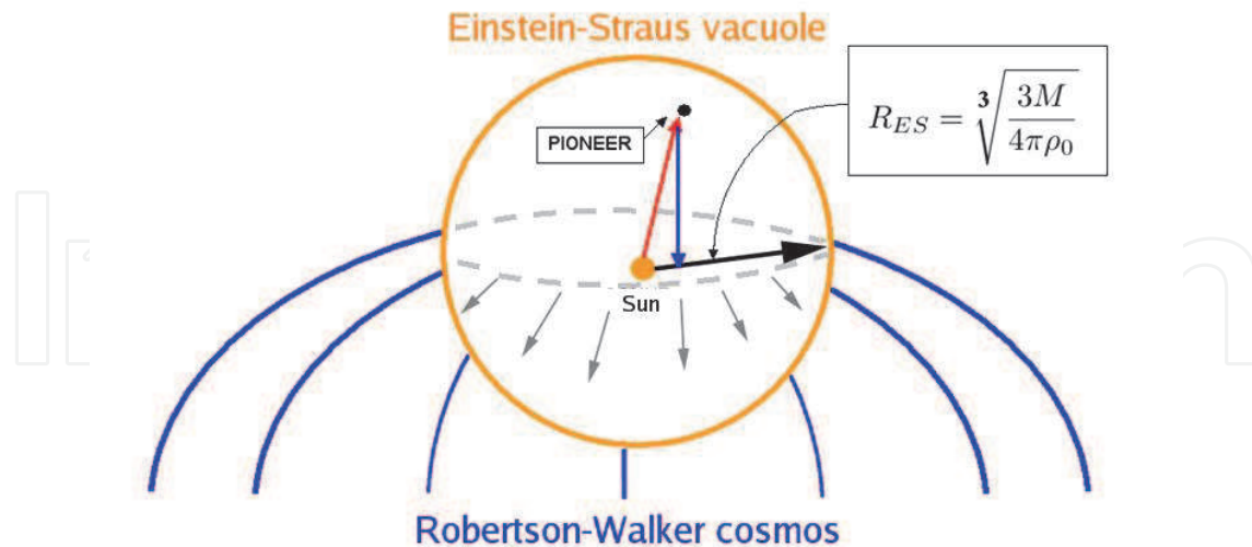
Fig. 2. Visualization of the Einstein-Straus globule surrounding a mass M within the expanding Robertson-Walker universe.
