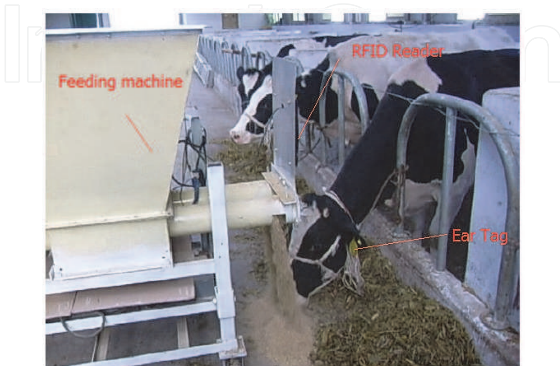
Fig. 9. Feeding Machine (Ni, 2009)
