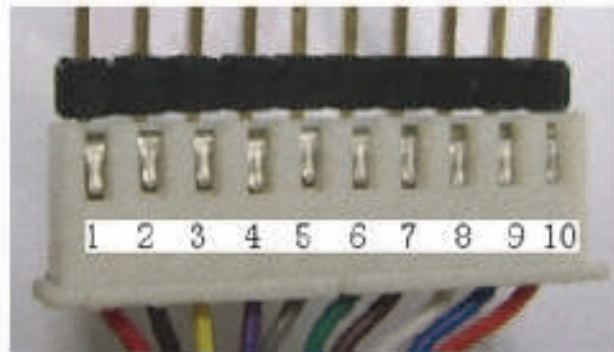
Fig. 6. I/O pins for SMC-R134 (Ni, 2009)
