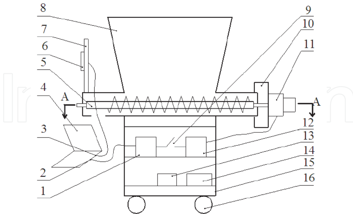
1-MCU, 2-First Serial Port, 3-Second Serial Port, 4-PC, 5-Auger, 6-RFID system, 7-Board for RFID, 8-Feed Bin, 9-Switch, 10-Board for Motor, 11-Motor, 12-Motor Actiyator, 13-Voltage Transfer Device, 14-Battery, 15-Frame, 16-Moving Device
