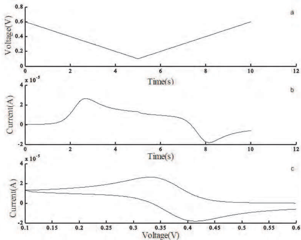
Fig. 2. (A) Applied voltage, (B) Measured current, (C) CV, combining (A) and (B).
