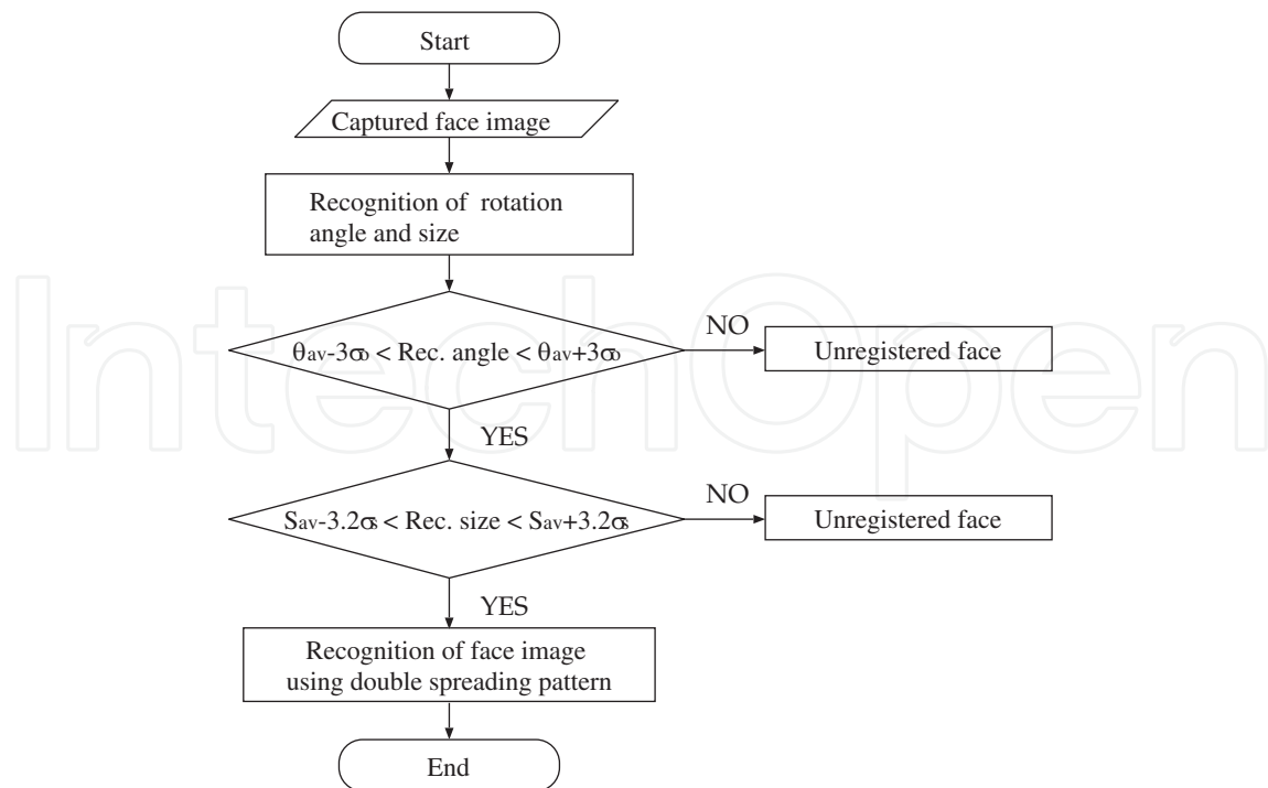
Fig. 13. Flowchart of new shape recognition process using the characteristics of orientation and size recognition.
