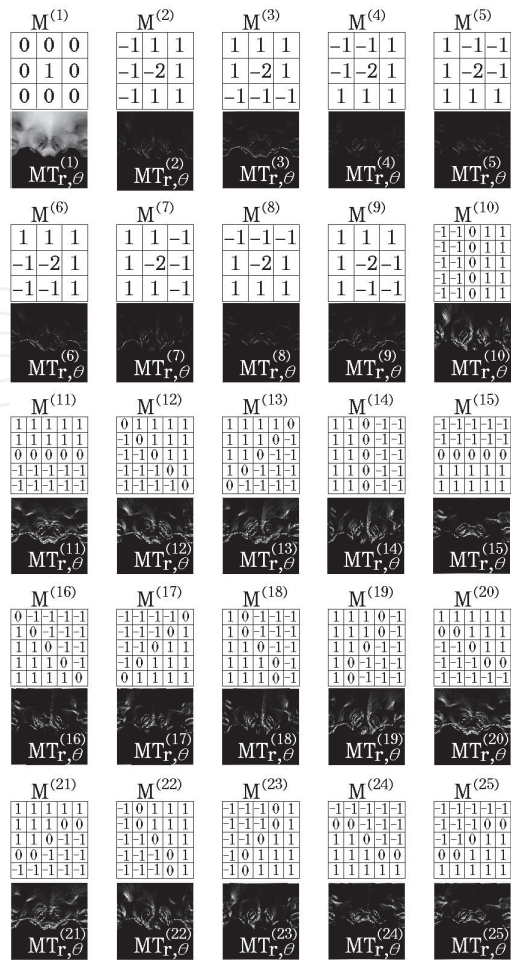
Fig. 2. Masks M^{(m)} and masked images MT_{r,\theta}^{(m)} .
