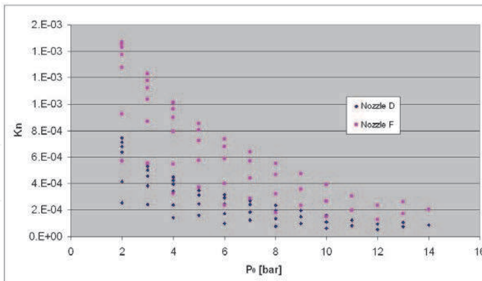
Fig. 1. Kn vs Reservoir pressure in Scirocco PWT.
