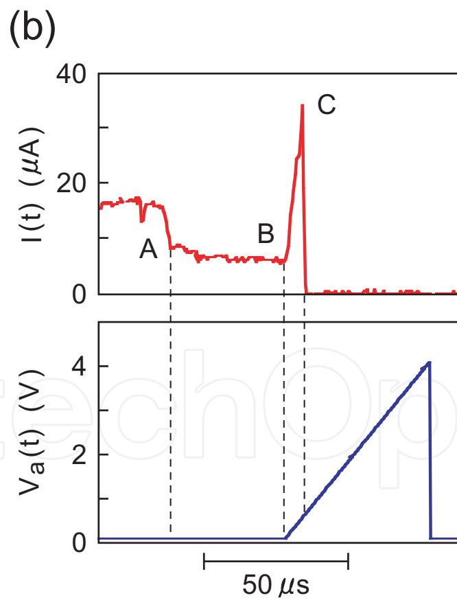
Fig. 11. Experimental setup (a) and typical temporal changes in the contact current and the bias voltage (b) in the break voltage measurements on an Au single-atom contact. See text for details.
