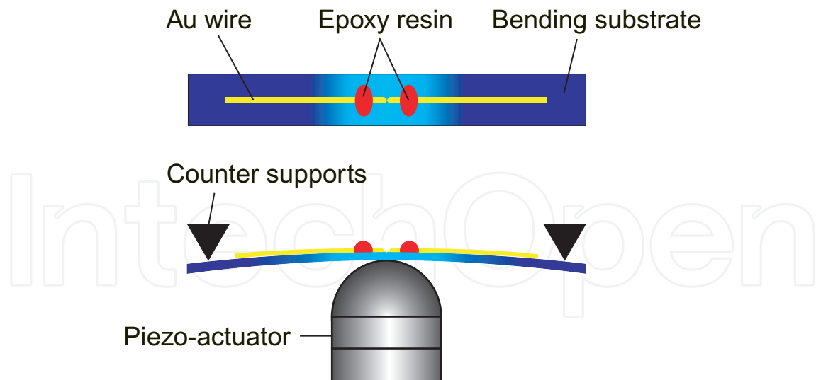
Fig. 4. Schematic of MCBJ (mechanically controllable break junction).
