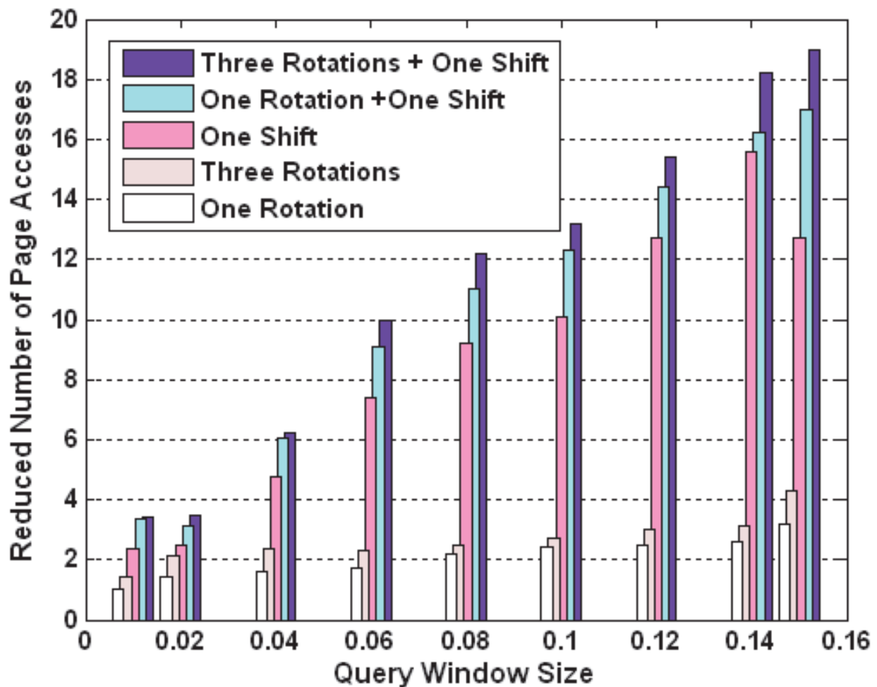
Fig. 10. Efficiency comparisons.
