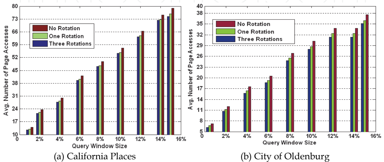
Fig. 8. Comparison of different rotations.
