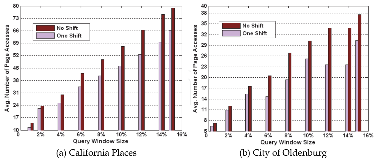
Fig. 9. Comparison on shift.
