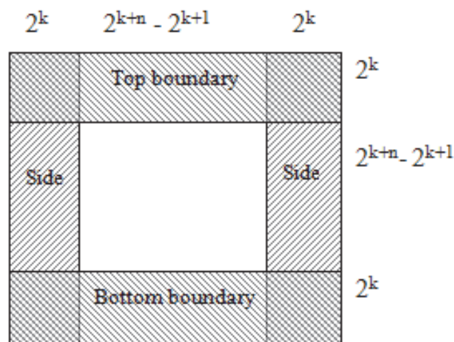
Fig. 4. H_{k+n} divided into 9 subregions.
