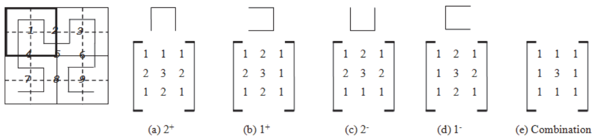
Fig. 2. Clusters with different orders.
