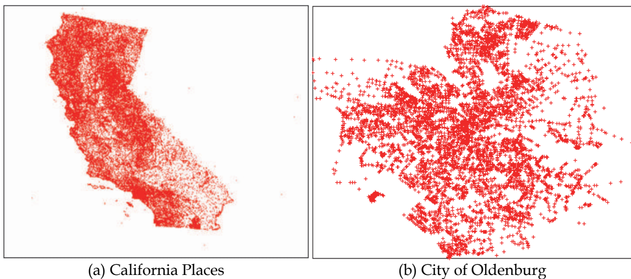
Fig. 6. Datasets.
