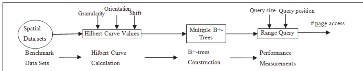
Fig. 7. Experimental design.
