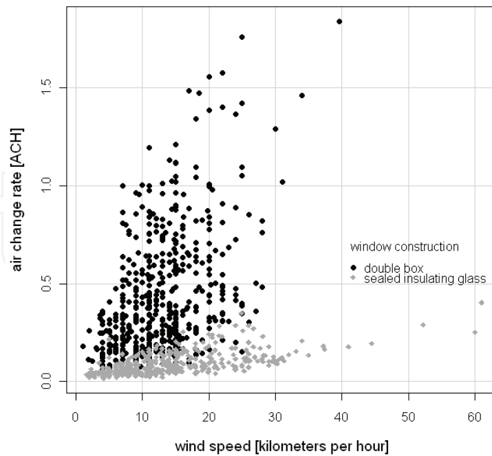
Fig. 11. Influence of wind speed on ACR in office spaces equipped with windows of different construction. Windows and doors closed. Rooms with double box windows (A-D, F: n= 611), room with insulating glass window: n= 388).
