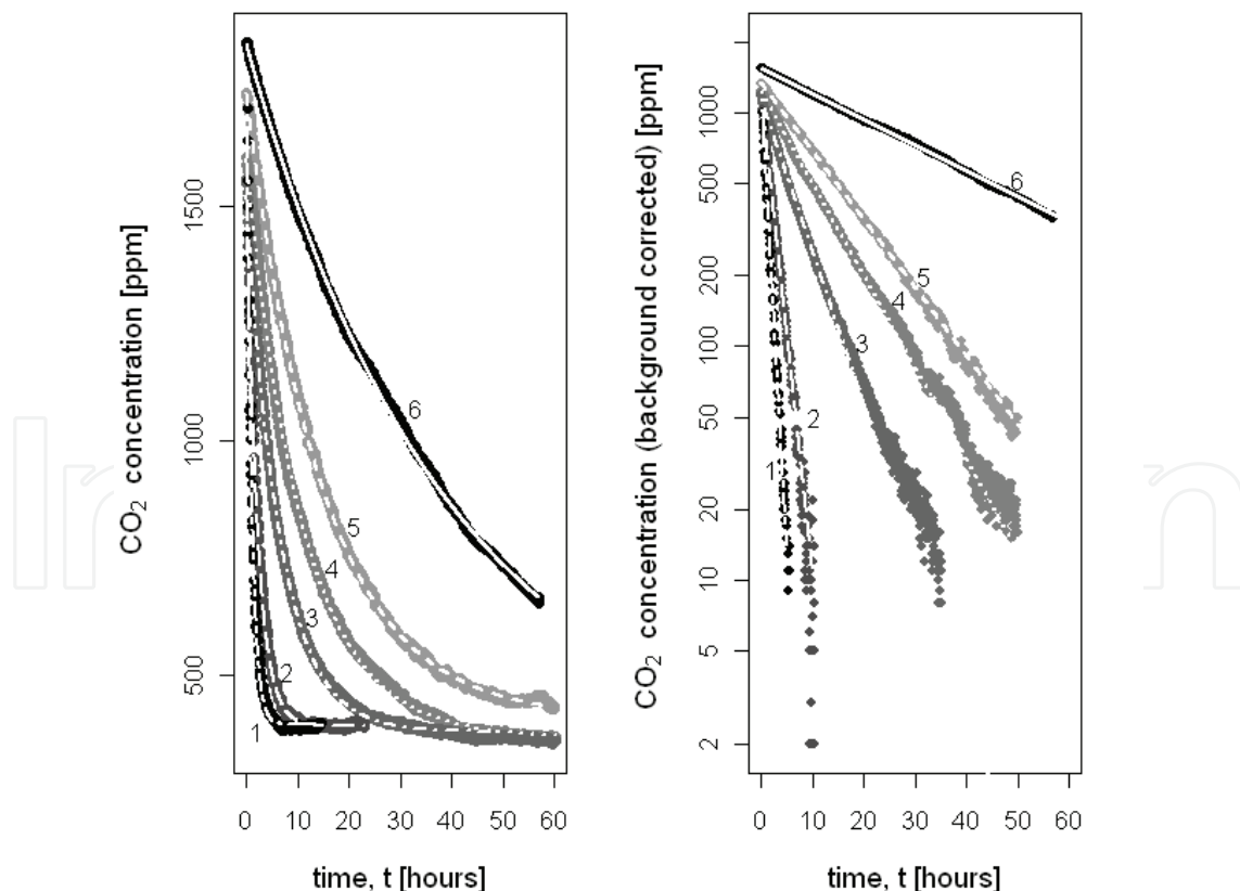
Fig. 5. CO 2 decay curves (black) in 6 rooms of different air tightness. White curves show results of regression analyses; a, nonlinear regression; b, linear regression of logarithmic values
