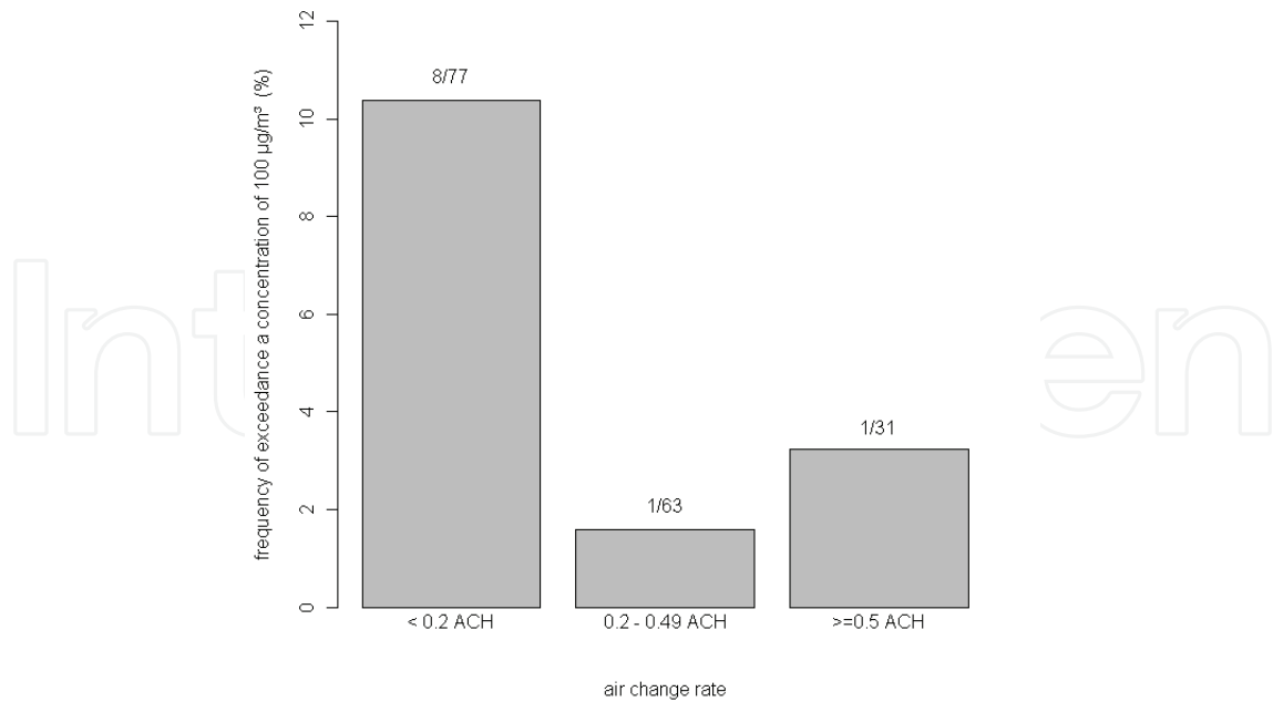
Fig. 16. Frequency of formaldehyde concentrations >100 \mu\text{g}/\text{m}^3 and ACR (natural ventilation) in rooms of the City of Berlin.
