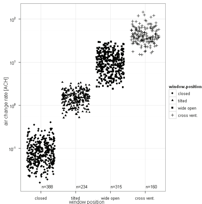
Fig. 13. ACR and window position. Office room E.
