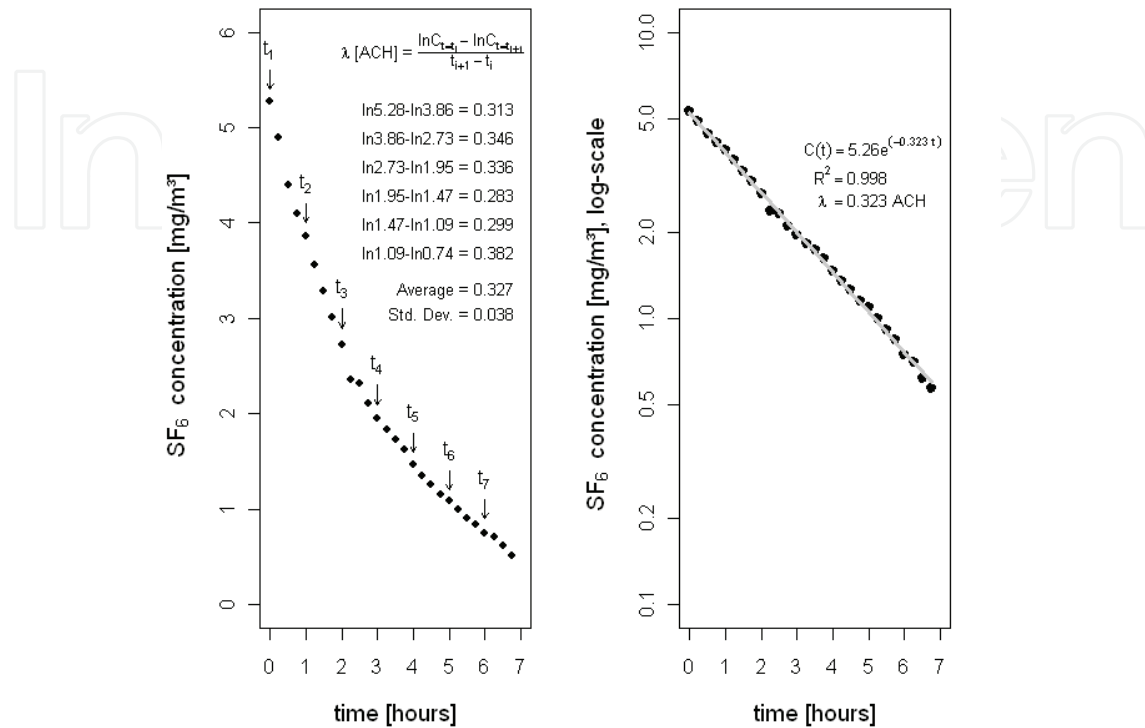
Fig. 2. ACR determination from concentration decay with the two-point method, time interval t_{i+1} - t_i between two measurements: one hour; a, linear scale; b, logarithmic scale, linear regression.
