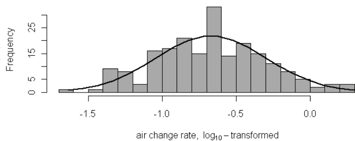
Fig. 15. Empirical frequency distribution of ACR (natural ventilation) for 198 rooms in the City of Berlin; a, values as determined; b, log-transformed values. Solid line represents normal distribution.
