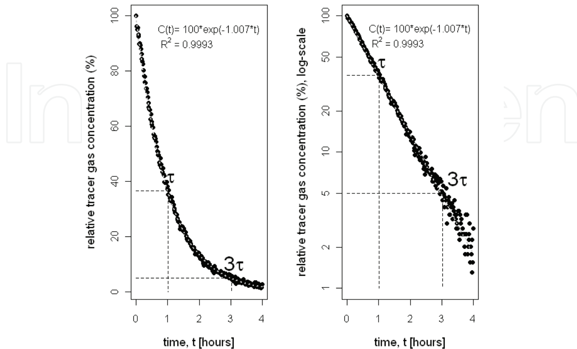
Fig. 1. Relationship between tracer gas concentration and time; a, untransformed ordinate; b, after logarithmic transformation.
