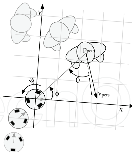
Fig. 2. The state variables p_{pers} and v_{pers} hold the position and velocity of the person in the robot's coordinate frame. \theta is the orientation of the person and \dot{\psi} is the rotational velocity of the robot.
