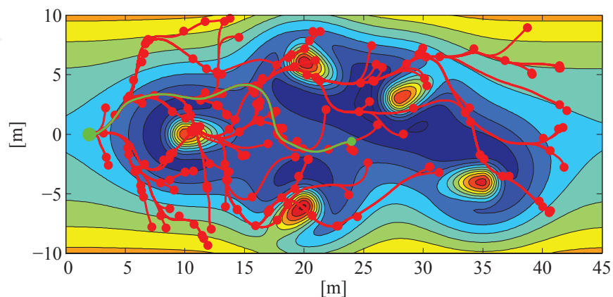
Fig. 12. An RRT for a robot starting at (2,0) and the task of moving forward through the human populated environment. Only every 10th vertex is shown to avoid clutter of the graph. The vertices are the red dots, and the lines are the simulated trajectories. The green trajectory is the least cost trajectory.
