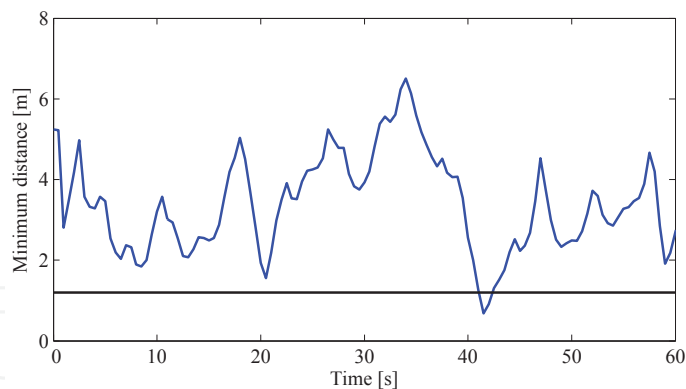
Fig. 14. The figure shows the closest distance of any person for one randomly chosen simulation. The horizontal black line, is at 1.2\text{m} distance, which corresponds to the transition between the social zone and the personal zone, which the robot should try to stay out of.
