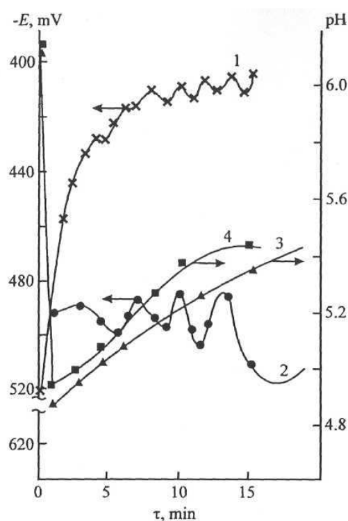
Fig. 6. Temperature dependencies of electrochemical potential (1, 2) and pH (3, 4) at 20 T (1, 3) and 40^\circ\text{C} (2, 4); 0.01 wt.% \text{H}_2\text{O}_2 .
