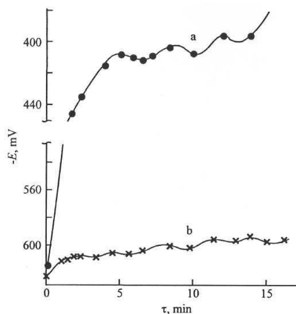
Fig. 5. The mixing effect on the change of electric potential in the system. T = 20^\circ\text{C} , 0.01 wt.% \text{H}_2\text{O}_2 (a: mixed system; b: without mixing).
