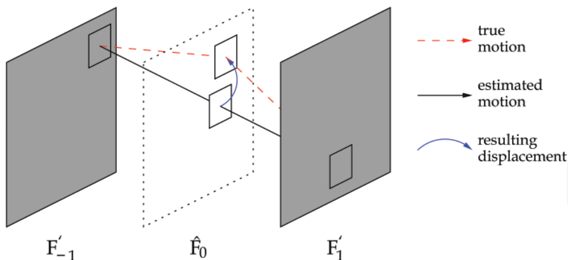
Fig. 7. Displaced interpolation due to nonlinear motion.
