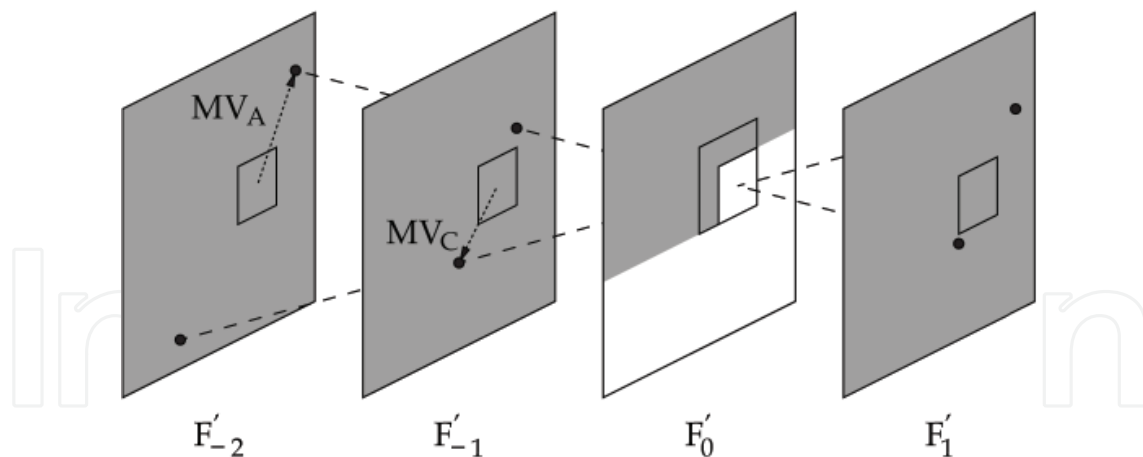
Fig. 5. L-shaped template used for motion search of the current block. Already decoded frame regions are shown in grey. The candidates (black circles) for template matching are derived from motion vectors of two neighbouring blocks ( MV_A , MV_C ) using linear scaling.
