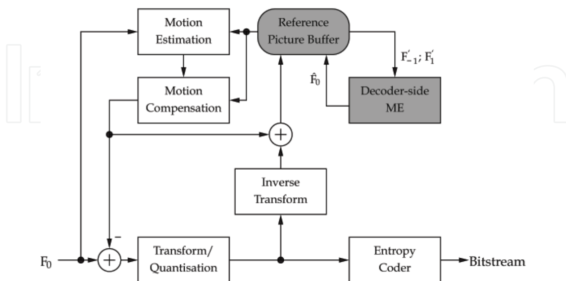
Fig. 6. Simplified block diagram of a conventional hybrid encoder with DSME modifications, as proposed by Klomp et al. (2009), highlighted in grey.
