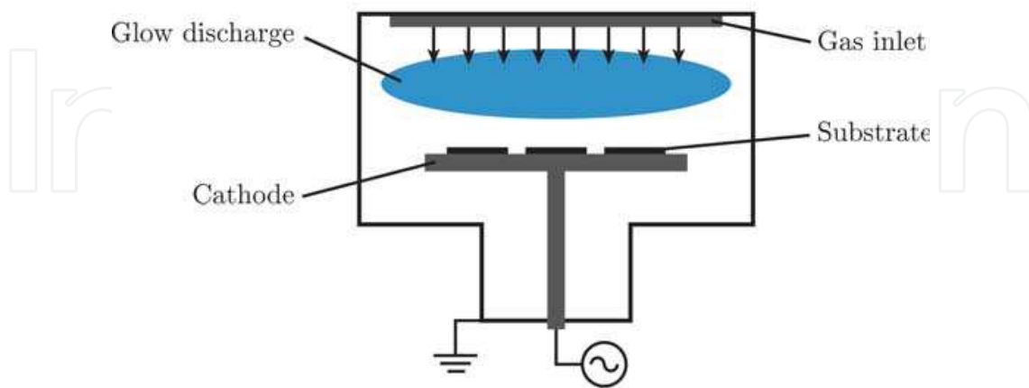
Fig. 2. Layout of a PECVD reactor.
