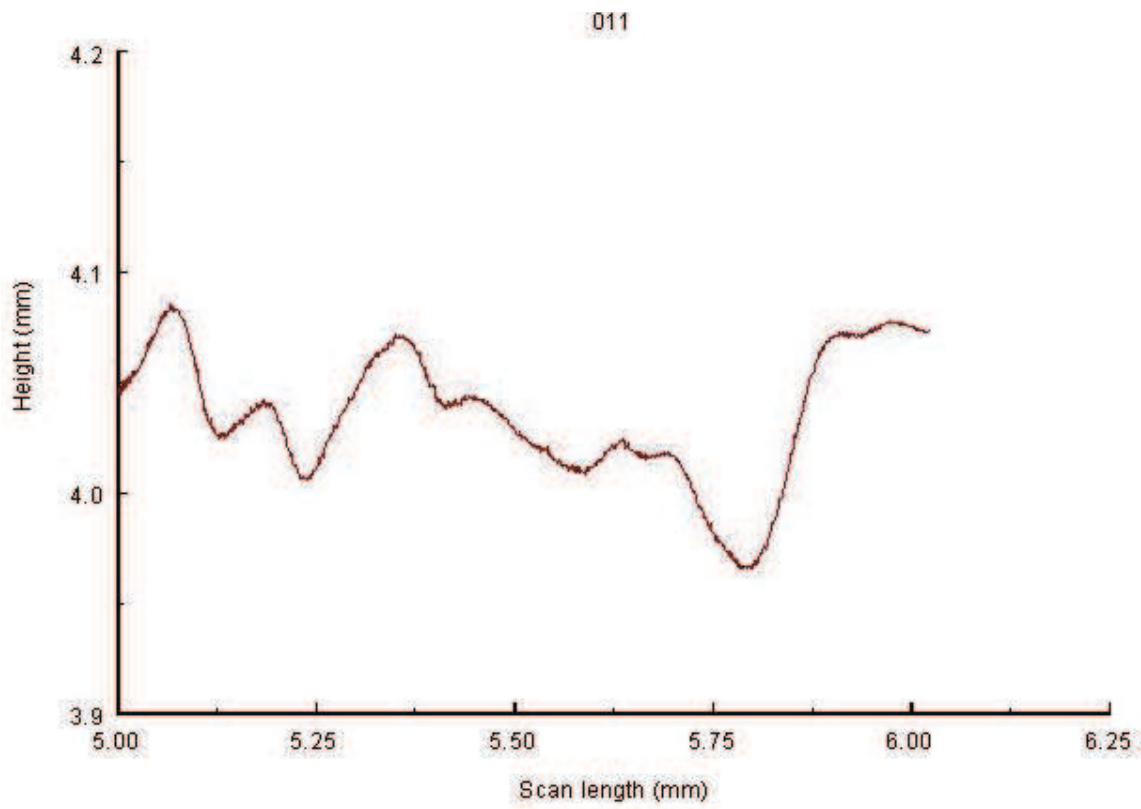
Fig. 2a. 1 micron scan from polished aggregate surface
