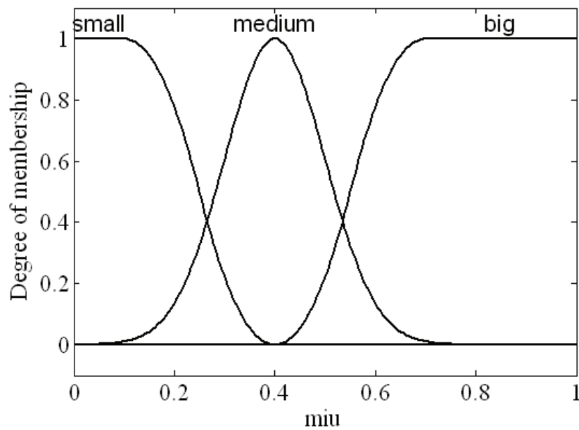
Fig. 3. Fuzzy membership function
