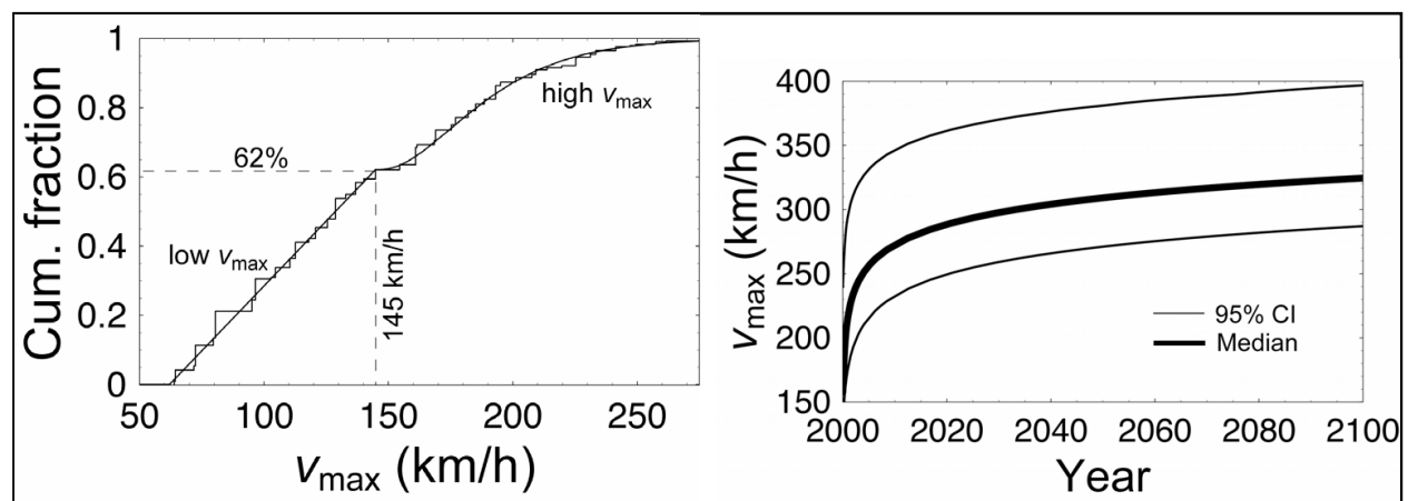
Fig. 5. (left) Cumulative empirical distribution of storm-specific v_{\max} , shown with a corresponding composite uniform-gamma distribution (solid line for low v_{\max} region, curve for high v_{\max} region). (right) Estimated median trend (bold curve) in \text{Max}(v_{\max}) extremes, v_m = \text{Max}(v_{\max}) | m with m = t-s for calendar year t and reference year s = 2000 , and corresponding 2-tail 95% confidence limits (light curves) predicted by the extreme-value model given by Eq. 3.
