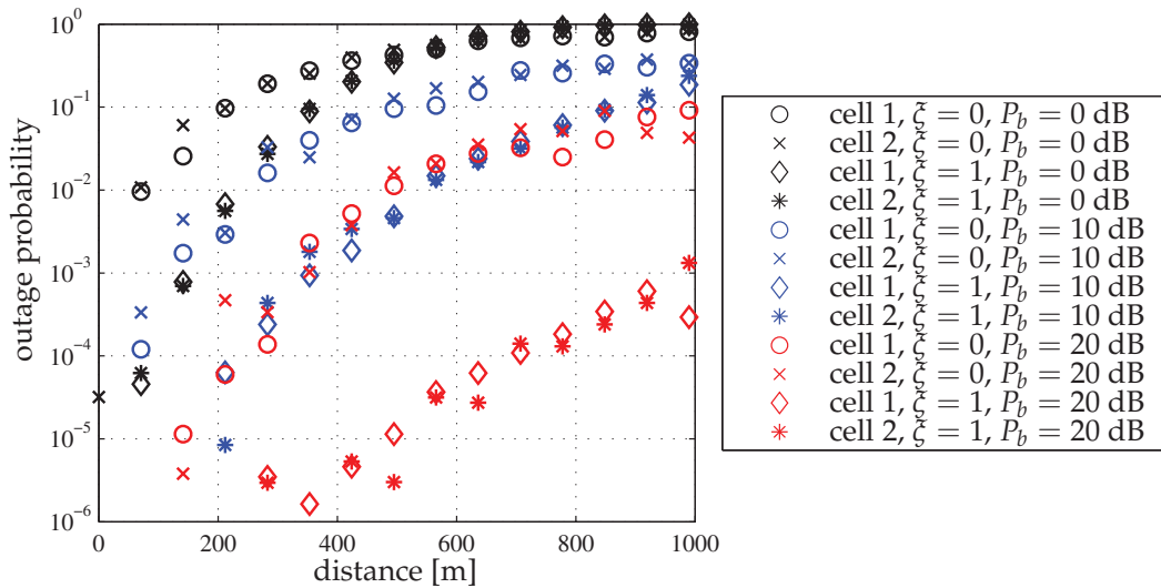
Fig. 6. Outage probability versus distance for given values of transmit power.
