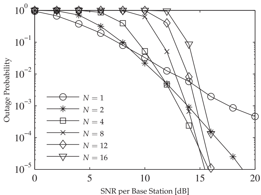
Fig. 8. Outage probability as a function of SNR
