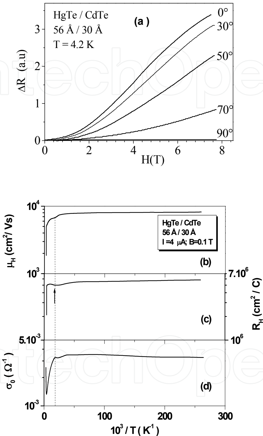
Fig. 5. (a) Variation of magnetoresistance of the sample with various angles between the magnetic field and the normal to the HgTe/CdTe superlattice surface. Temperature dependence of the Hall mobility (b), weak-field Hall coefficient (c) and conductivity (d) (Nafidi et al, 2002) in the investigated HgTe/CdTe superlattice
