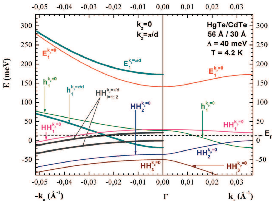
Fig. 4. Calculated bands along the wave vector k_z in the right and in plane k_p(k_x, k_y) in the left, of the HgTe/CdTe superlattice at 4.2 K. E_F is the energy of Fermi level
