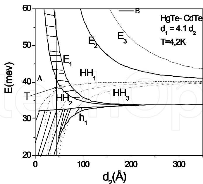
Fig. 8. Energy position and width of the conduction ( E_n ), heavy-hole ( \text{HH}_n ), and the first light-hole ( h_1 ) subbands calculated at 4.2 K in the center \Gamma of the first Brillion zone as a function of layer thickness d_2 for HgTe/CdTe superlattice with d_1 = 4.1 d_2 . T is the point of the transition semiconductor- semimetal
