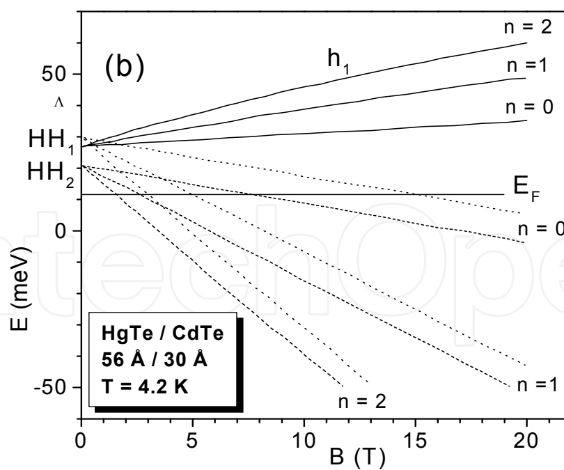
Fig. 6. (a) Variation of transverse magnetoresistance, with magnetic field of HgTe/CdTe superlattice, at 4.2 K (b) calculated Landau levels as a function of applied magnetic field of the HgTe/CdTe SL at 4,2 K. E_F is the Fermi level energy
