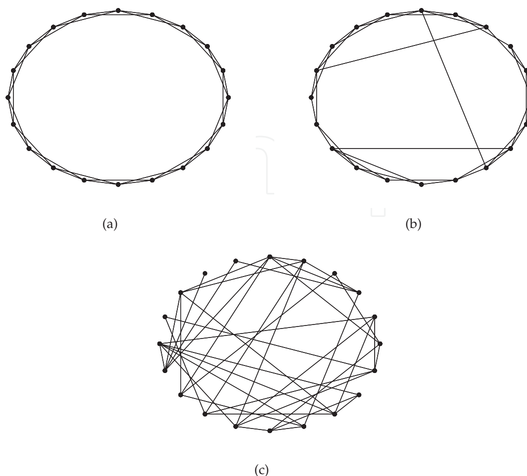
Fig. 1. Procedure of redirection of links in a regular network (a) with increasing probability p . As p increases the network moves from regular (a) to random (c), becoming small world (b) for a critical value of p . n=20, k=4
