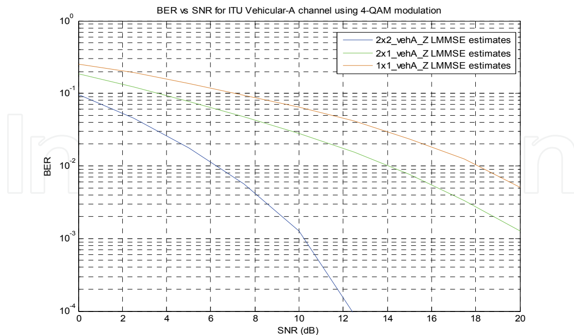
Fig. 9. BER performance of LTE transceiver with multiple antennas for ITU Vehicular-A channel model using 4-QAM modulation and LMMSE channel estimation
