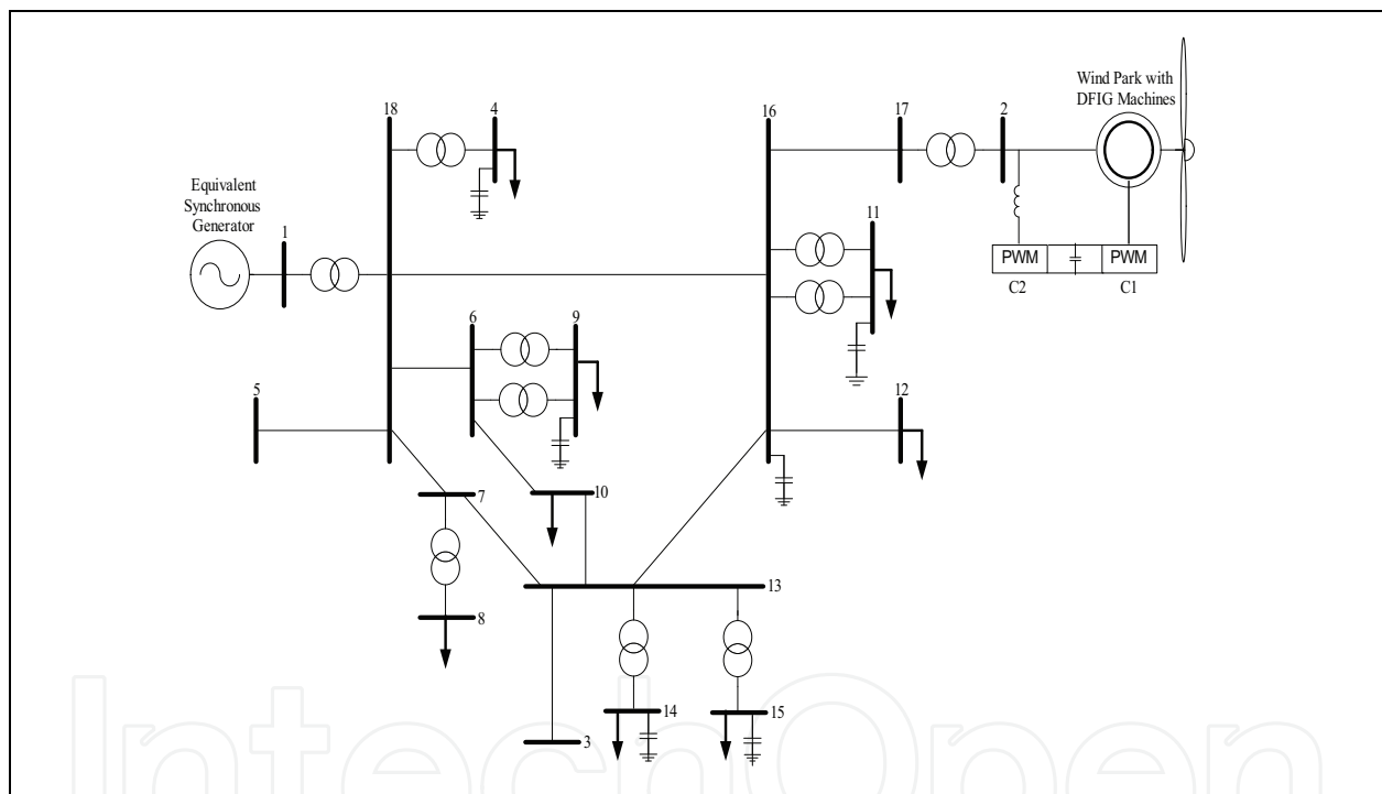
Fig. 2. Electrical Network
