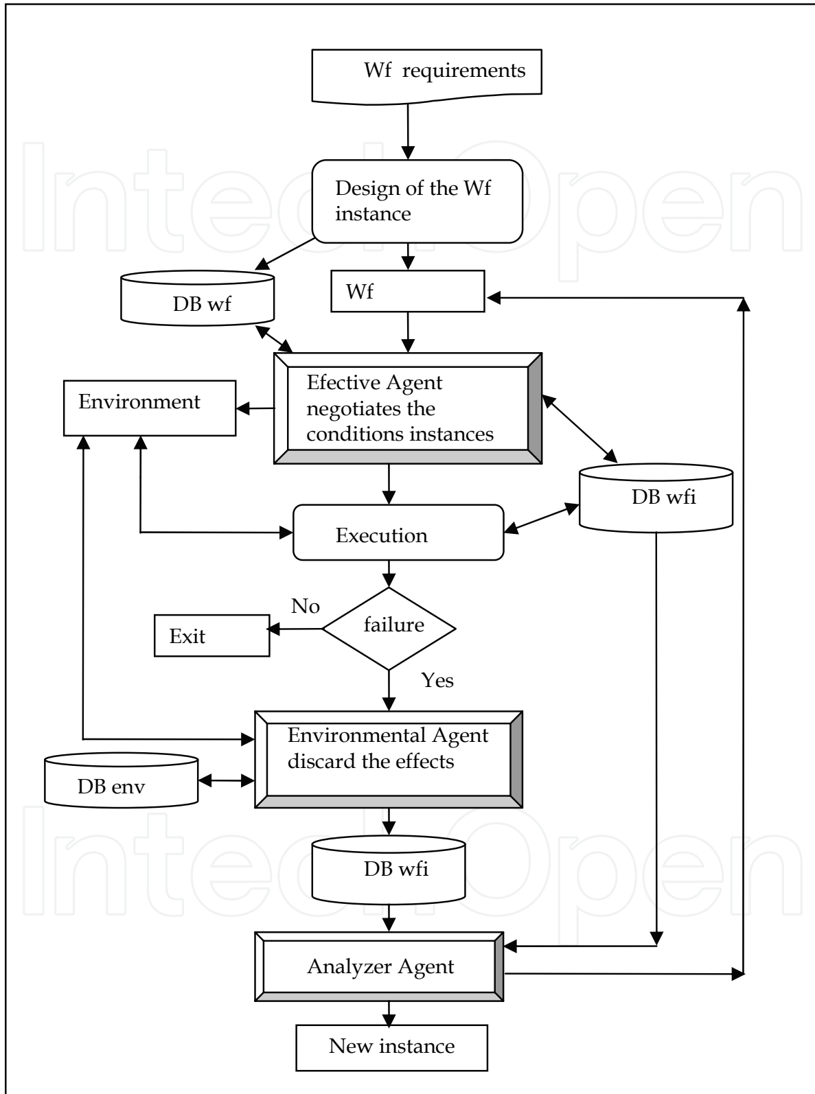
Fig. 8. Interaction of the agents with data bases
