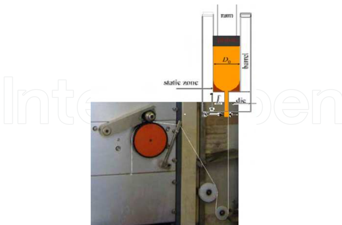
Fig. 1. Scheme of apparatus for filament formation
