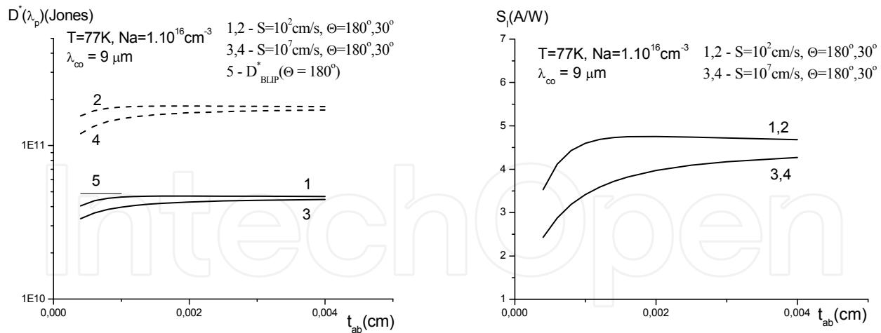
Fig. 5. Calculated peak detectivity D^*(\lambda_p) and peak responsivity S_l(\lambda_p) of \text{Hg}_{0.766}\text{Cd}_{0.234}\text{Te} photodiodes with n^+ - p junction versus thickness of p -absorber t_{ab} at \text{FOV}=180^\circ - (1 and 3) and \text{FOV}=30^\circ - (2 and 4). Surface recombination rate s=10^2 \text{ cm/sec} (1 and 2) and s=10^7 \text{ cm/sec} (3 and 4). Operating temperature 77 K. Background temperature equals to 293 K. Doping of p -absorber p_{77}=10^{16} \text{ cm}^{-3} , n^+ - p junction area 20 \mu\text{m} \times 20 \mu\text{m}
