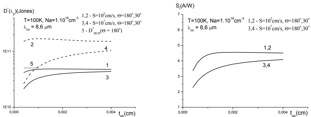
Fig. 6. Calculated peak detectivity D^*(\lambda_p) and peak responsivity S_l(\lambda_p) of \text{Hg}_{0.766}\text{Cd}_{0.234}\text{Te} photodiodes with n^+ - p junction versus thickness of p -absorber t_{ab} at \text{FOV}=180^\circ - (1 and 3) and \text{FOV}=30^\circ - (2 and 4). Surface recombination rate s=10^2 \text{ cm/sec} (1 and 2) and s=10^7 \text{ cm/sec} (3 and 4). Operating temperature 100 K. Background temperature equals to 293 K. Doping of p -absorber p_{77}=10^{16} \text{ cm}^{-3} , n^+ - p junction area 20 \mu\text{m} \times 20 \mu\text{m}
