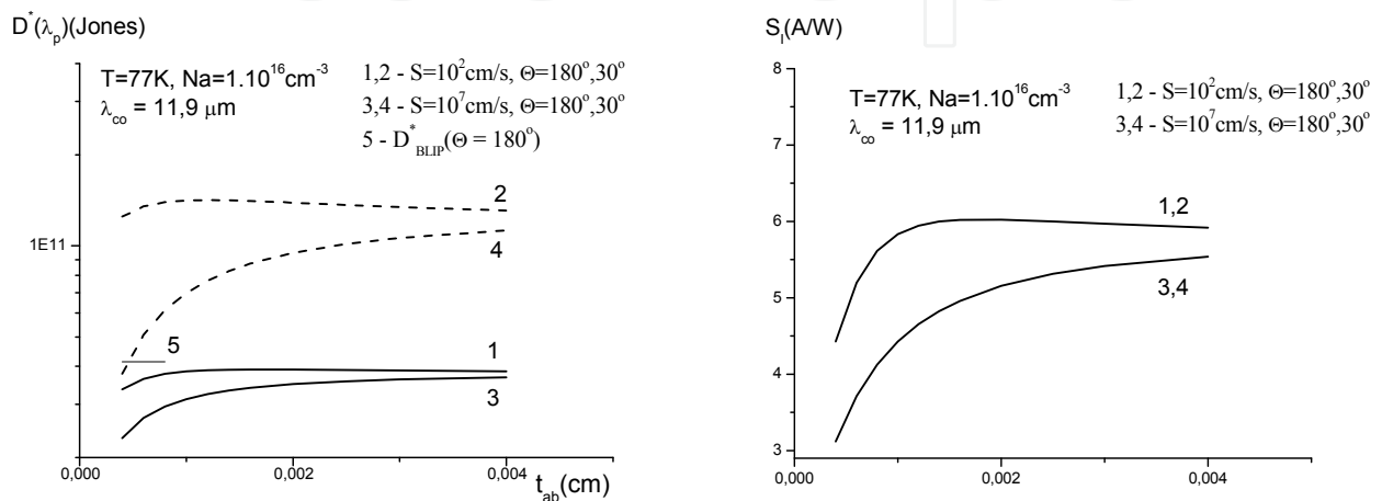
Fig. 1. Calculated peak detectivity D^*(\lambda_p) and peak responsivity S_l(\lambda_p) of Hg_{0.785}Cd_{0.215}Te photodiodes with n+-p junction versus thickness of p-absorber t_{ab} at FOV=180 ^\circ - (1 and 3) and FOV=30 ^\circ - (2 and 4). Surface recombination rate s=10^2 cm/sec (1 and 2) and s=10^7 cm/sec (3 and 4). Operating temperature 77 K. Background temperature equals to 293 K. Doping of p-absorber p_{77}=10^{16} cm ^{-3} , n+-p junction area 20 \mu m \times 20 \mu m
