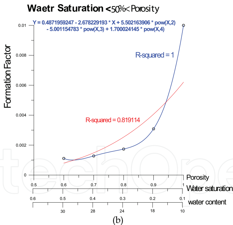
Fig. 5. Analytical relationship between Formation factor, porosity, water saturation and water content in the two different cases.
