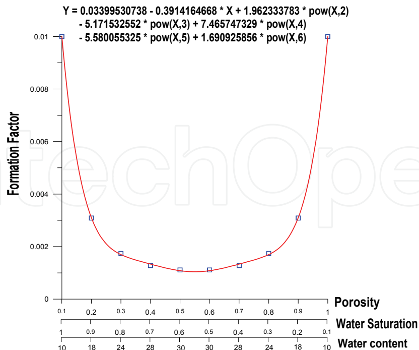
Fig. 4. Analytical relationship between Formation factor, porosity, water saturation and water content when porosity \neq water saturation.
