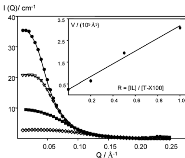
Fig. 2. SANS from single-phase [\text{h-bmim}][\text{BF}_4] in cyclohexane- d_{12} microemulsions at 55^\circ\text{C} . R = 0 ( \diamond ), 0.2 ( \blacksquare ), 0.5 ( \triangle ), and 1.0 ( \bullet ); \phi_{\text{T-X100}} = 0.41 . The fits shown as lines are to a form factor for homogeneous ellipsoids. Inset shows the micelle swelling behavior in terms of the ellipsoid volume V as a function of added IL. (Reproduced from (Eastoe et al., 2005), with permission, copyright American Chemical Society, 2008).
