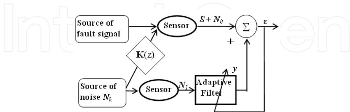
Fig. 6. Adaptive noise cancelling
