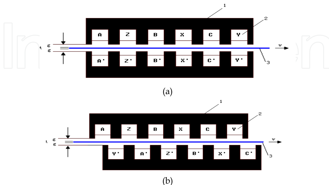
Fig. 9. (a) Schematic of a typical double-sided TWIHI system; (b) Schematic of the double-sided C-TWIHI system (1-magnetic yoke; 2-exciting windings; 3-load metal sheet; t -strip thickness; g -airgap between inductor and load; v -strip movement velocity. Phase degree: A-X and A'-X'=0^\circ , B-Y and B'-Y'=-120^\circ , C-Z and C'-Z'=-240^\circ ).
