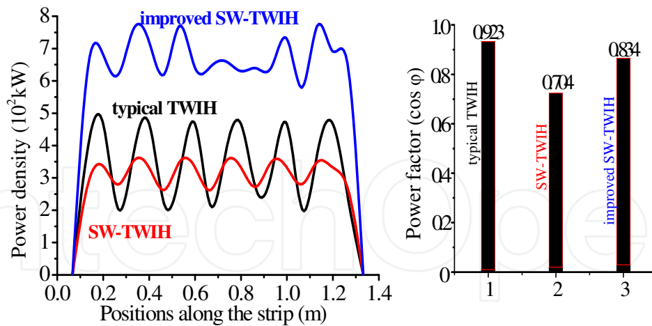
Fig. 21. Relative power density distributions and the power factor.
