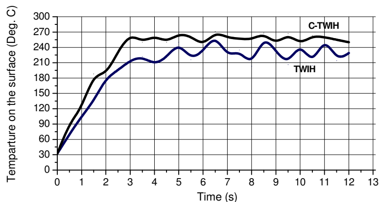
Fig. 16. Temperature distribution along the surface of the strip
