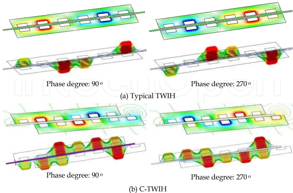
Fig. 13. Magnetic flux distributions in the strip and induced power density distributions along the direction of the strip movement (yoke size - 1300×30mm; slot size - 150 ×50 mm; airgap - 1 mm; strip thickness - 2 mm; currents supply I -1200A; f - 600 Hz).
