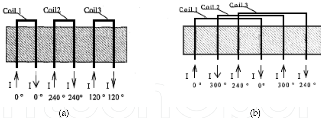
Fig. 6. (a) Coil connections for TFIH; (b) Coil connections for TWIH.
