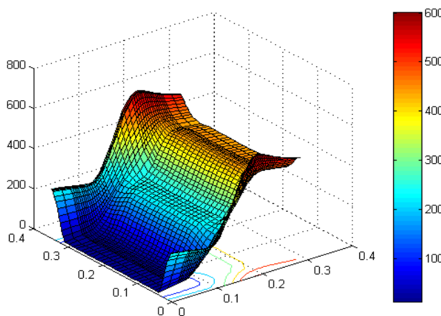
Fig. 3. Temperature distribution on the surface of the strip
