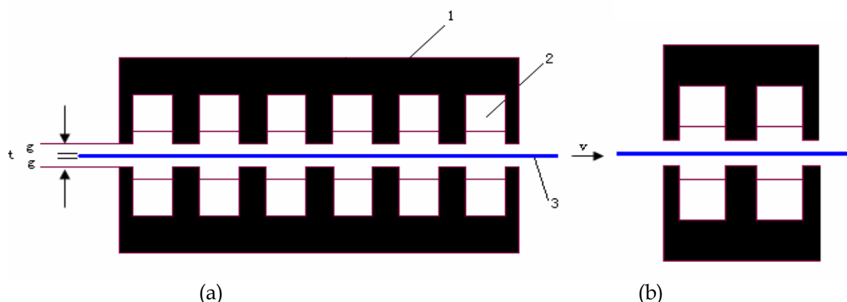
Fig. 5. (a) Schematic of a double-side TWIH [1-magnetic yoke; 2-exciting windings; 3-load metal sheet; t-strip thickness; g-airgap between inductor and load; v-strip movement directions]; (b) Schematic of a double-side TFIH.
