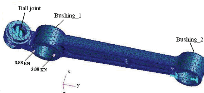
Fig. 7. Finite element model of the lower suspension arm
