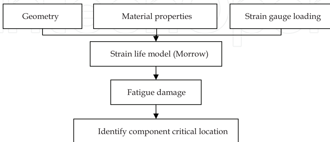
Fig. 11. Schematic diagram of calculating fatigue damage values for the collected loadings
