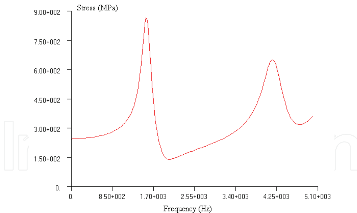
Fig. 15. Automobile lower suspension arm stress plotted against frequency (0-5000 Hz)
