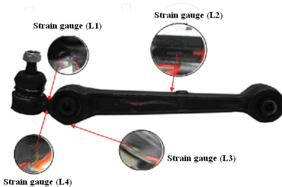
Fig. 9. The strain gauge positions on the lower suspension arm
