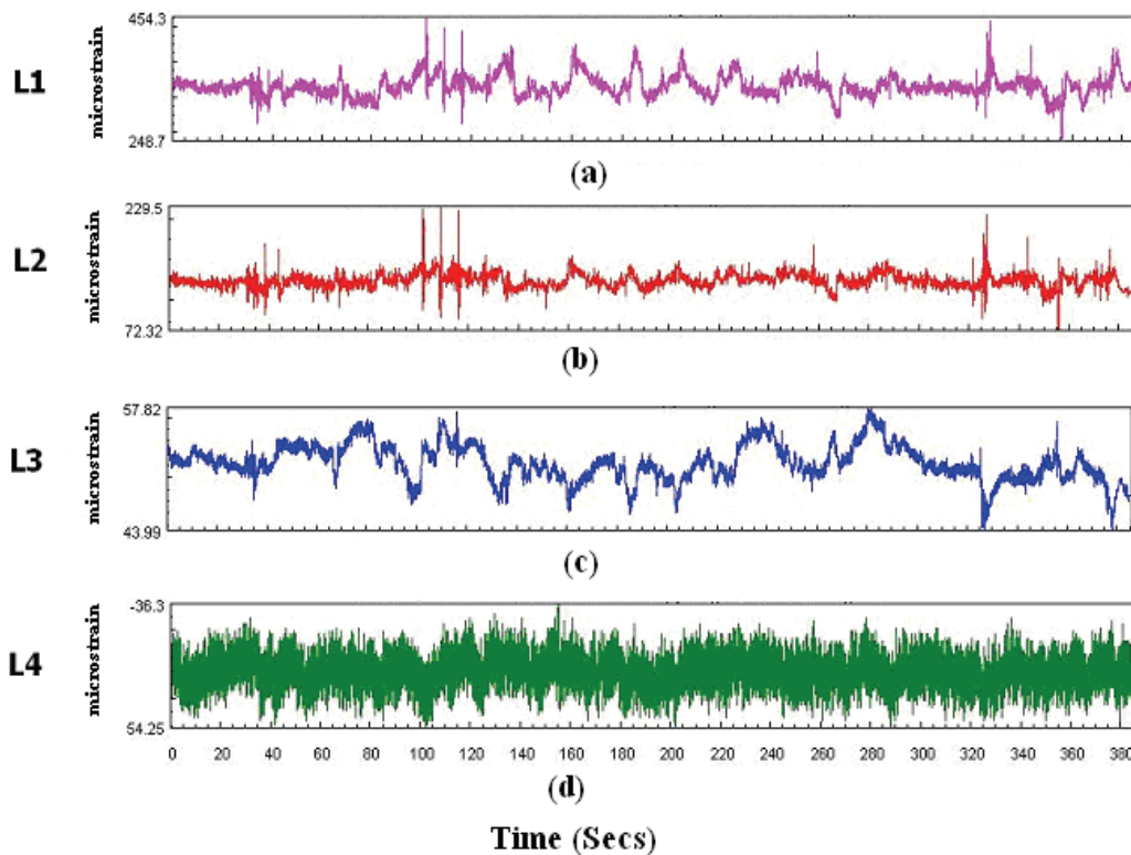
Fig. 10. Strain time history plot for different strain gauge positions: (a) L1, (b) L2, (c) L3, (d) L4
