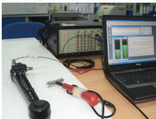
Fig. 6. The set up of data acquisition Portable Analyser Pulse to be used for normal mode analysis test
