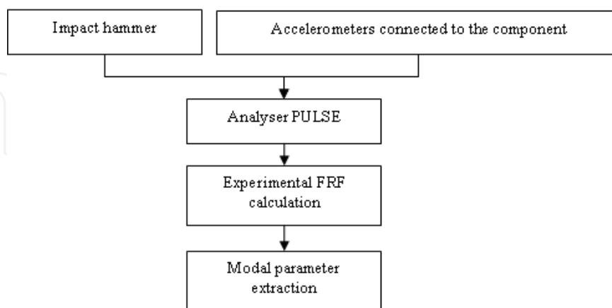
Fig. 5. Schematic diagram of experimental modal test
