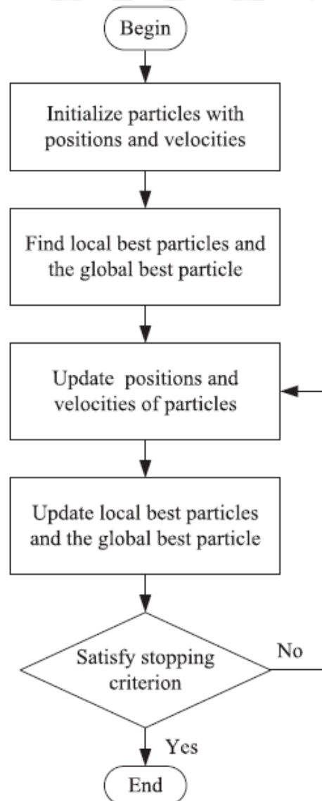
Fig. 7. Flowchart of the PSO algorithm [27].
