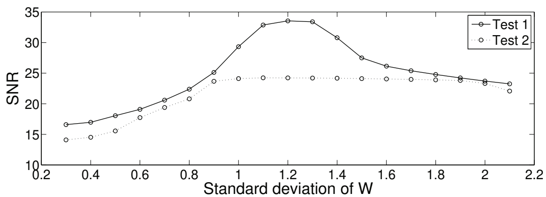
Fig. 3. Influence of W on fusion performance.
