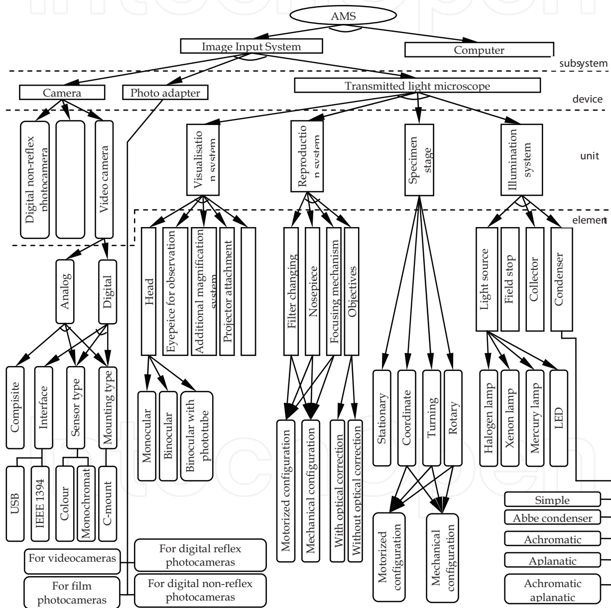
Fig. 4. AND-OR tree of hardware part of AMS
