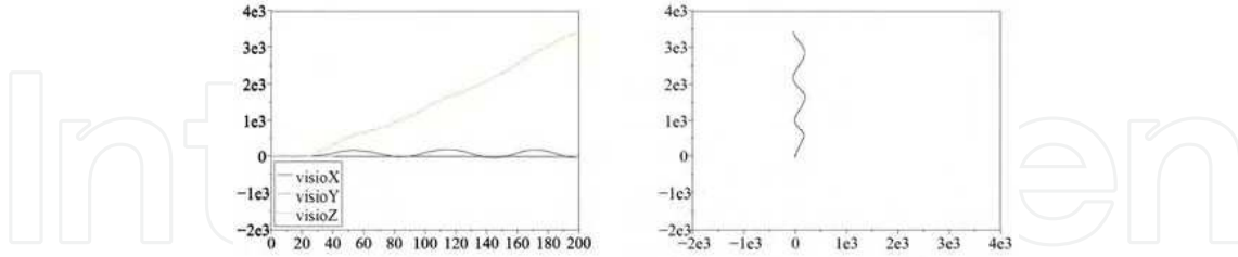
Fig. 7. (a) Evolution of the recovered T_x , T_y and T_z components (in millimeters). (b) Computed trajectory (in millimeters) in the XZ plane.
