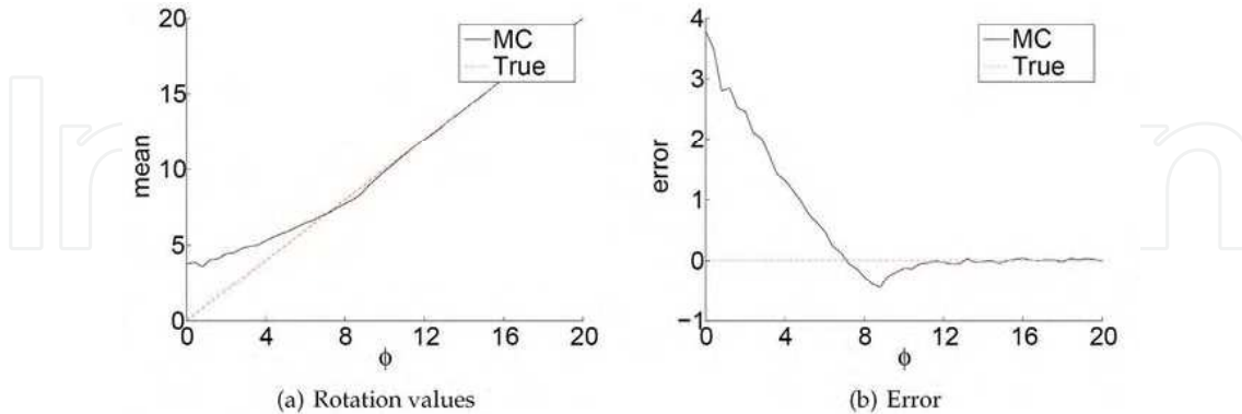
Fig. 2. Systematic error in the R_x component. Continuous line for values obtained with Monte Carlo simulation and dotted line for true values. The same is applicable to the R_y component.
