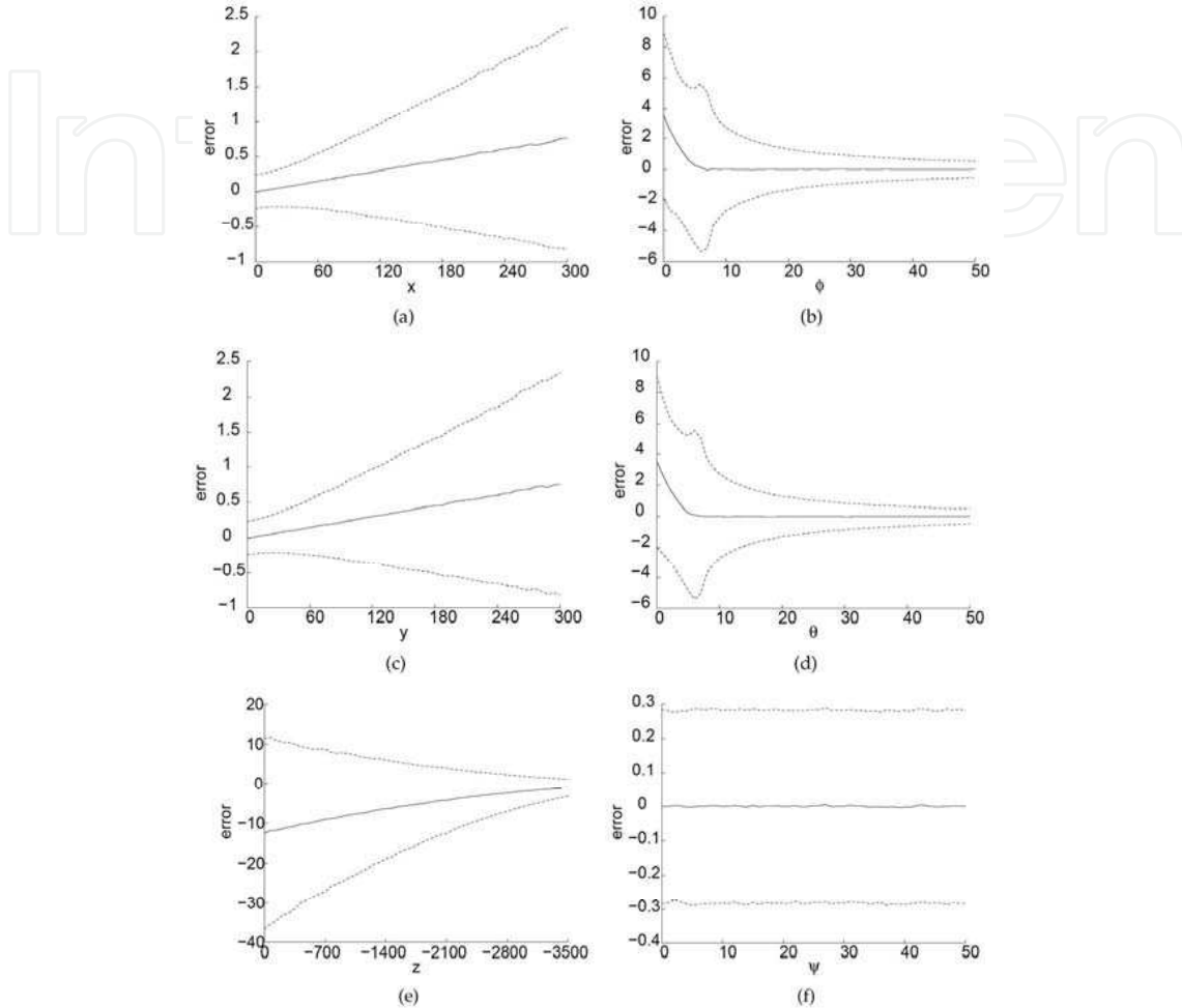
Fig. 4. Mean error (solid lines) and 2\sigma deviation (dashed lines) for pure motions along and about the 6 coordinate axes of a camera placed at 5000mm and focal length 50mm . Errors in T_x and T_y translations are equivalent, small while centered and increasing while uncentered, and translation is worst recovered for T_z (although it gets better while approximating). Errors for small R_x and R_y rotations are large, as contour deformation in the image is small, while for large transformations errors are less significant. The error in R_z rotations is negligible.
