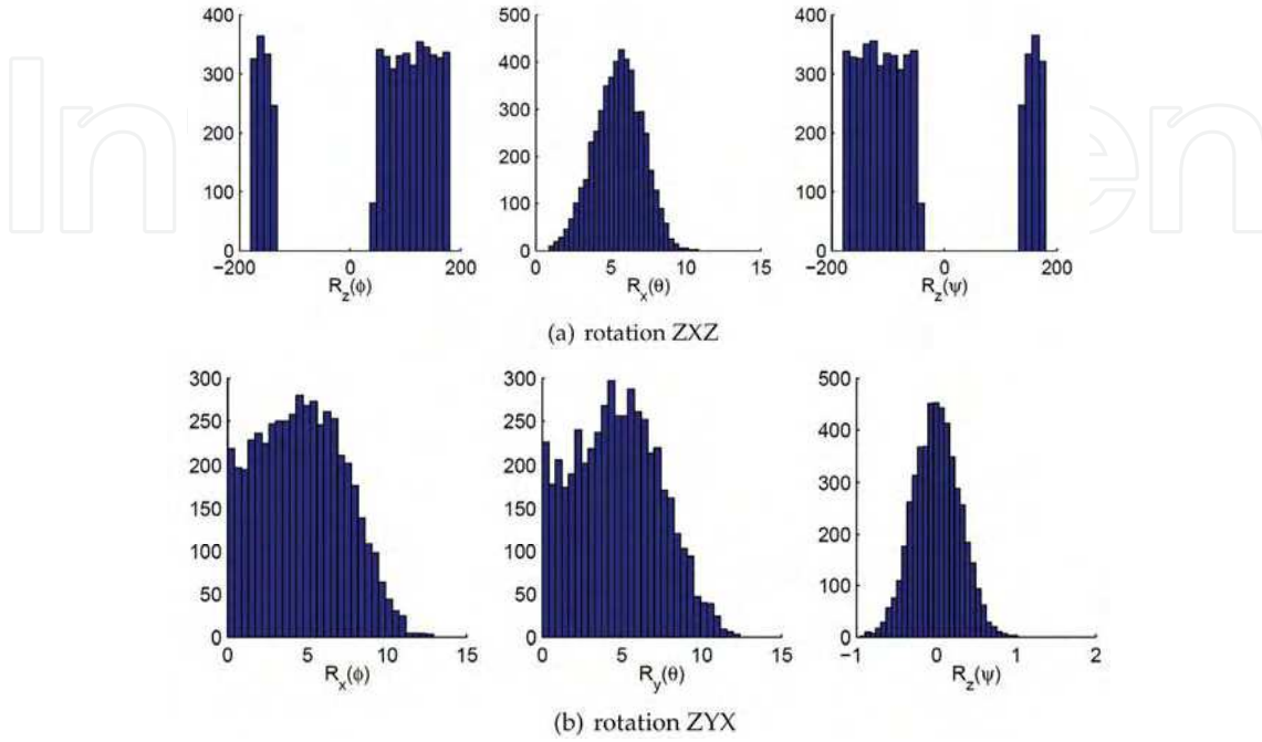
Fig. 1. Histogram of the computed rotation values for 5000 trials adding Gaussian noise with \sigma = 0.5 pixels to the contour control points. (a) In the ZXZ representation, small variations of the pose correspond to discontinuous values in the rotation components R_z(\phi) and R_z(\psi) . (b) In contrast, the same rotations in the ZYX representation yield continuous values.
