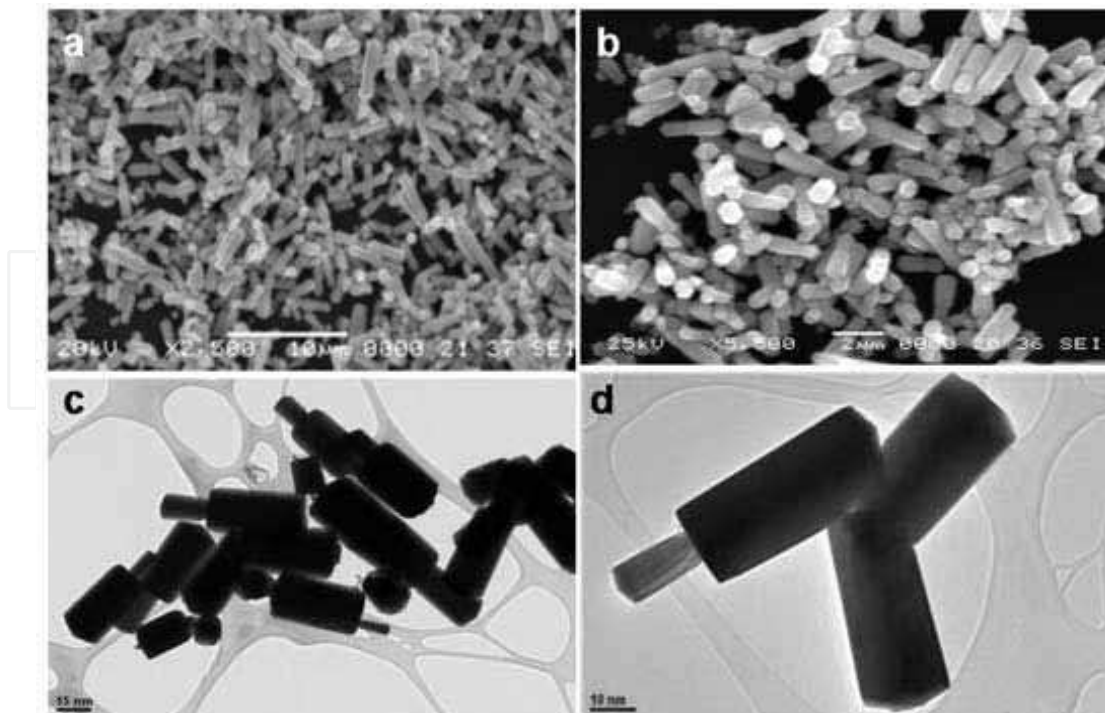
Fig. 8. (a and b) Scanning electron micrograph of ZnO nanorods. (c and d) Transmission electron micrograph of ZnO nanorods.
