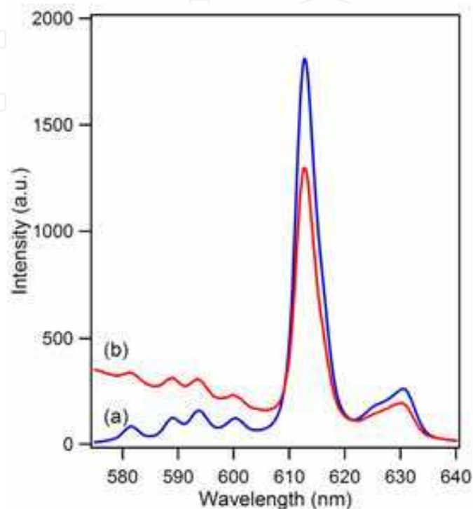
Fig. 7. Photoluminescence spectra comparison of \text{Eu}^{3+} doped \text{Gd}_2\text{O}_3 nanotubes (a) and nanorods (b) annealed at 600\text{ }^\circ\text{C} , respectively.
